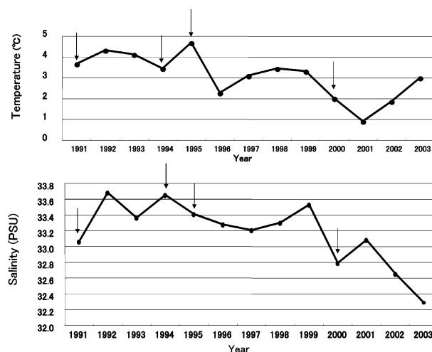
Fig. 5. Annual fluctuation of temperature and salinity at a depth of 15 m in mid February at Station 30 (Station 26 in 1991) from 1991 to 2003. Arrows indicate the years occurring the strong year classes.
