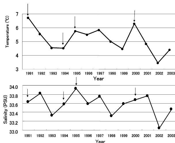
Fig. 4. Annual fluctuation of temperature and salinity at a depth of 15 m in late January at Station 30 from 1991 to 2003. Arrows indicate the years occurring the strong year classes.
