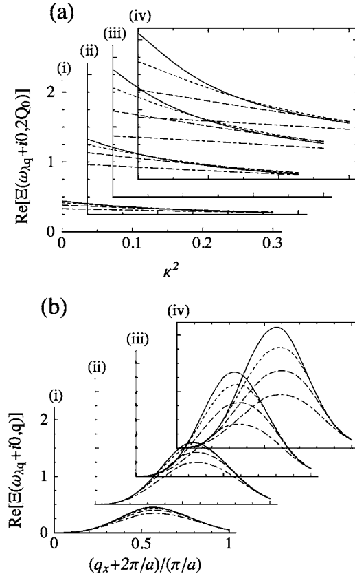
FIG. 1. (a) \text{Re}[\Xi(\omega_{\lambda q} + i0, 2\mathbf{Q}_0)] as a function of \kappa^2 , with \mathbf{Q}_0 = (-3\pi/4a, \pi/a) , and (b) \text{Re}[\Xi(\omega_{\lambda q} + i0, \mathbf{q})] as a function of q_x ( -2\pi/a \leq q_x \leq -\pi/a ) for q_y = 2\pi/a . For the anisotropy factor, (i) \delta=1 , (ii) \delta=10^{-1/2} , (iii) \delta=10^{-1} , and (iv) \delta=10^{-3} . In each figure, solid, dotted, dashed, and dashed chain lines are for \omega_{\lambda q}/\Gamma_{\text{AF}}=0.2, 0.4, 0.8 , and 1.6 , respectively.
