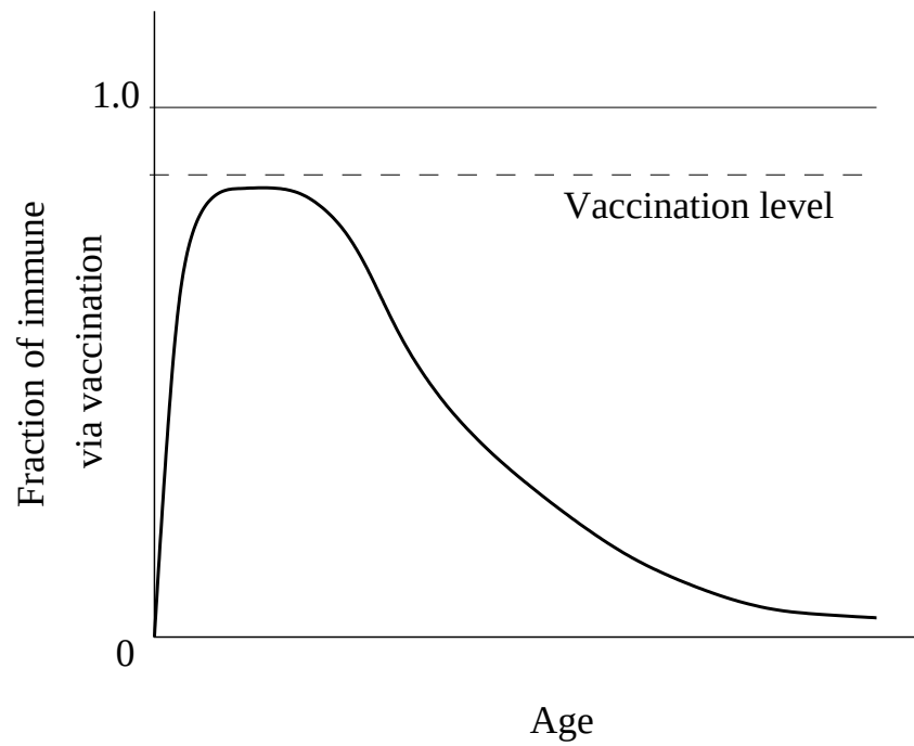
Fig. 1. Schematic distribution of population preserving immunity acquired through vaccination.
