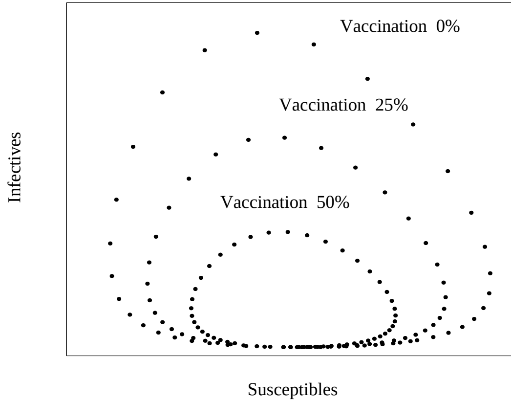
Fig. 3. Typical phase orbits of the system (1) for different vaccination rates and the same initial conditions (here b = 1/480 and R_0 = 16 ).
