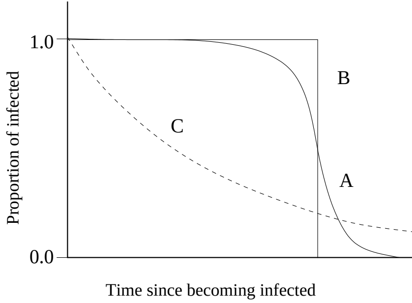
Fig. 2. Schematic representation of recovery. Here the curve A is for observed data, the curve B is for recovery of all infected after a definite period of time (a parasite generation) and the curve C is for continuous-rate recovery. A model has a basic reproductive number R_0 proportional to the area under the curve.
