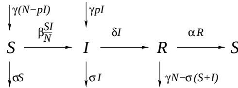
FIGURE 1. Transfer diagram of the SIRS model.
