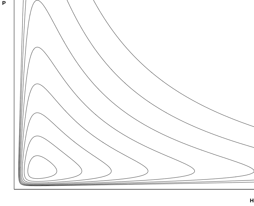
Fig. 1. Level curves of the Lyapunov function V(H, P) .
