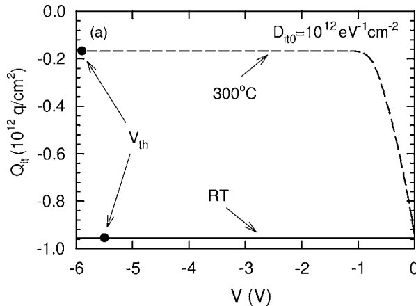
FIG. 8. (a) Dependence of the \text{SiN}_x/\text{AlGaIn} interface state charge ( Q_{it} ) vs gate bias in the MISH diodes at RT (solid line) and at 300^\circ\text{C} (dashed line). The threshold voltages ( V_{th} ) are indicated for both curves. The interface state density distribution was assumed to be as shown in Fig. 3(b) with D_{it0}=10^{12} \text{eV}^{-1} \text{cm}^{-2} . (b) Schematic view of the \text{SiN}_x/\text{AlGaIn} interface at RT for a gate bias slightly below zero and without electron emission from the interface states beneath the zero gate bias Fermi level ( E_{F0} ). The filled circles represent occupied states, and the empty circle the unoccupied state. (c) A similar view at 300^\circ\text{C} . The arrows indicate the electron emission from the interface states to the \text{AlGaIn} conduction band.
