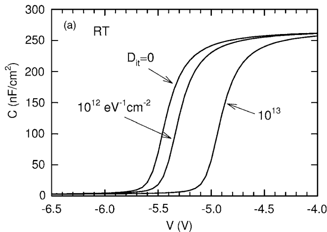
FIG. 6. Theoretical C - V curves calculated for the MISH capacitor with the \text{SiN}_x/\text{AlGaIn} interface state density distribution, as shown in Fig. 3(b), and various interface state density minima D_{it0} (a) at RT and (b) at 300 °C.
