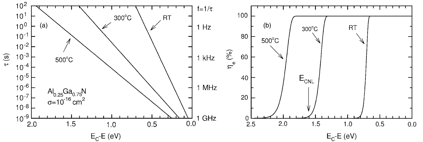
FIG. 2. (a) Time constant of electron emission from the interface traps to the \text{Al}_{0.25}\text{Ga}_{0.75}\text{N} conduction band and (b) emission efficiency vs trap energy at RT, 300 °C, and 500 °C. Parameters for the calculation were taken from Table I.
