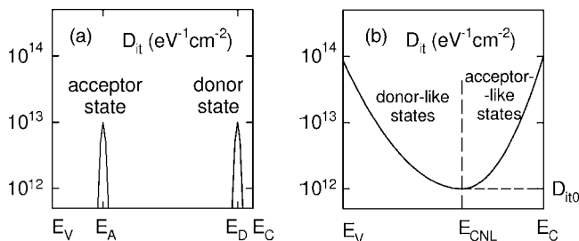
FIG. 3. \text{SiN}_x/\text{AlGaN} interface state density distribution used in the calculations: (a) the Gaussian peaks at E_A = E_V + 1 \text{ eV} and at E_D = E_C - 0.3 \text{ eV} and (b) the U-shaped distribution with E_{CNL} at 1.6 eV below E_C .
