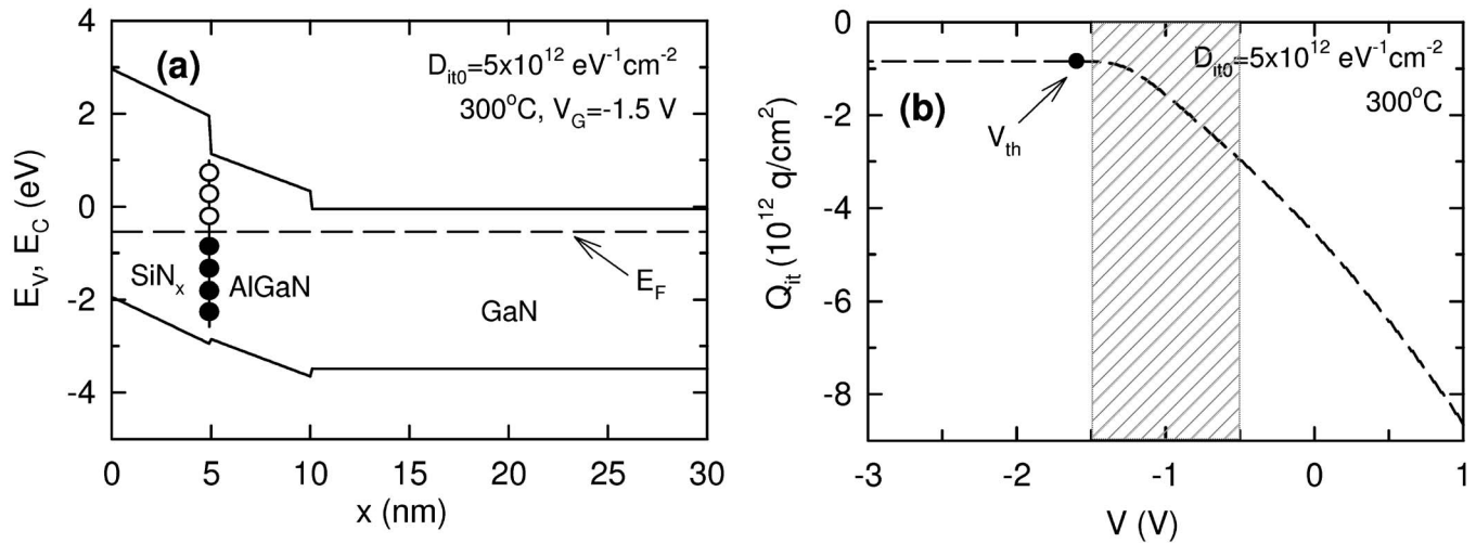
FIG. 12. (a) Band diagram of a MISH capacitor like that in Fig. 11(a) calculated at a bias slightly above the threshold voltage at 300 °C. The SiN x /AlGaIn interface state density distribution was assumed to be like that in Fig. 3(b) with D_{it0}=5 \times 10^{12} \text{ eV}^{-1} \text{ cm}^{-2} . (b) Dependence of the SiN x /AlGaIn interface state charge ( Q_{it} ) vs gate bias related to the dashed C - V curve from Fig. 11(b). The region of capacitance sensitivity to gate bias is marked as in Fig. 11(b) and the threshold voltage ( V_{th} ) is indicated.
