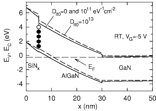
FIG. 7. Band diagrams of the \text{SiN}_x/\text{AlGaIn}/\text{GaN} structure calculated at a bias of -5 V (slightly above the threshold) at RT. The \text{SiN}_x/\text{AlGaIn} interface state density distribution was assumed to be like that of Fig. 3(b) with D_{it0}=0 , 10^{11} , and 10^{13} \text{eV}^{-1} \text{cm}^{-2} .
