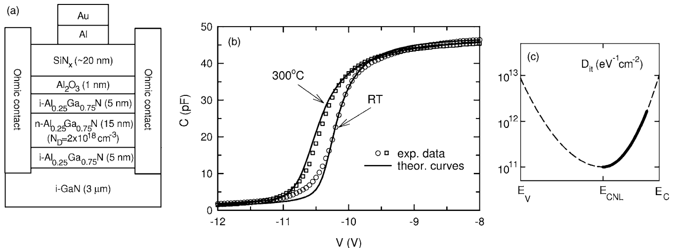
FIG. 13. (a) Schematic diagram of the fabricated SiN x /Al 2 O 3 /AlGaIn/GaN structure. (b) Experimental C - V characteristics from the MISH capacitor measured at RT (circles) and 300 °C (squares) and fitted theoretical curves (lines). (c) D_{it}(E) assumed in the calculation of the best fitted curve. The part of D_{it}(E) actually determined from the fitting is shown by the bold solid line.
