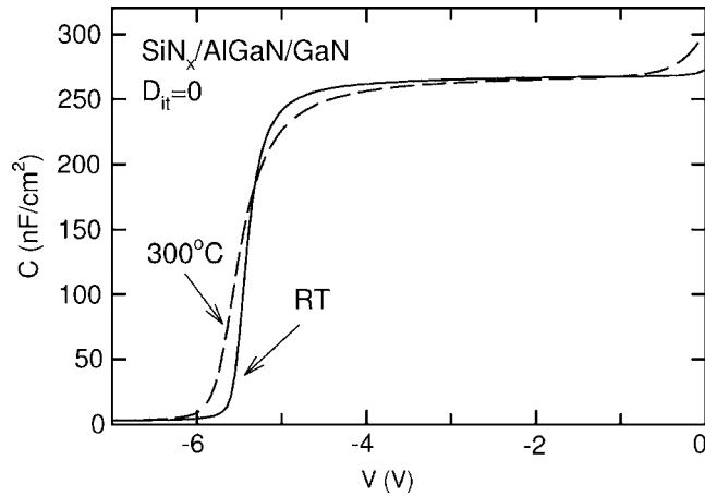
FIG. 4. Theoretical C - V curves calculated for a \text{SiN}_x/\text{AlGaIn}/\text{GaN} structure like that in Fig. 1 without interface states at RT (solid line) and at 300 °C (dashed line).
