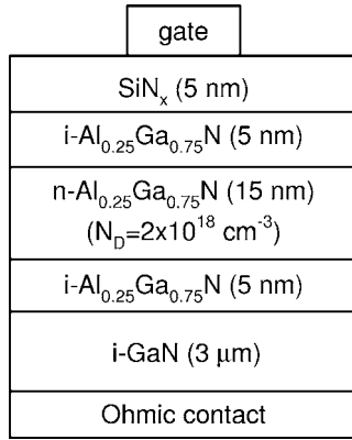
FIG. 1. Model structure used in the calculations.
