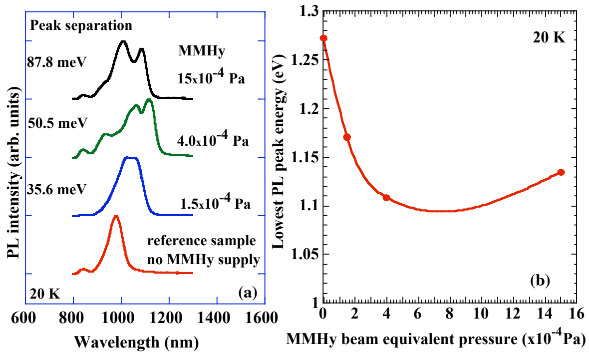
Fig. 1. (a) PL spectra of InAs QDs and their dependence on MMHy supply. (b) MMHy BEP dependence of QD lowest-state PL peak energies.
