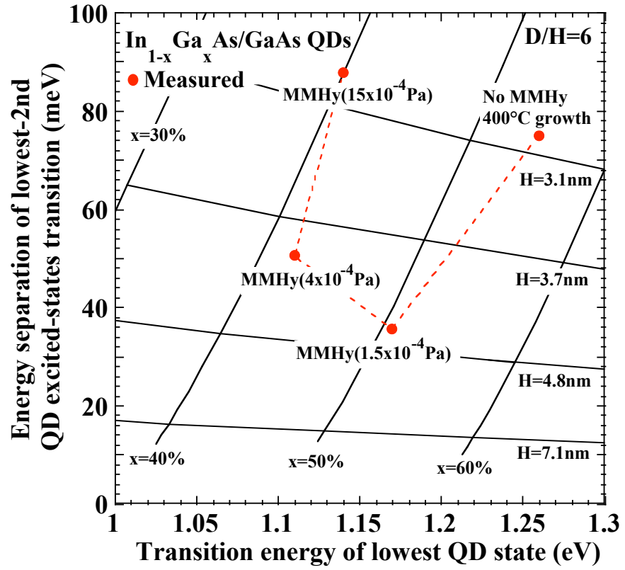
Fig. 4. Comparison of calculated relation between transition energy of lowest QD states and energy separation of lowest and second QD excited-state transitions with measurements.
