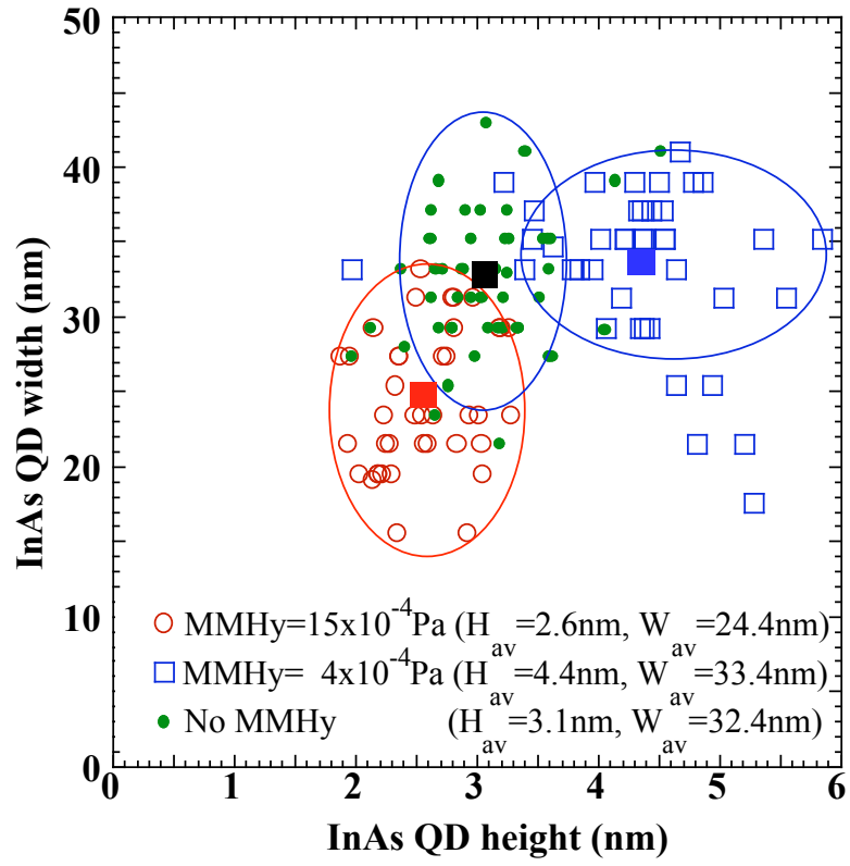
Fig. 3. InAs QD size distributions and their dependence on MMHy supply.
