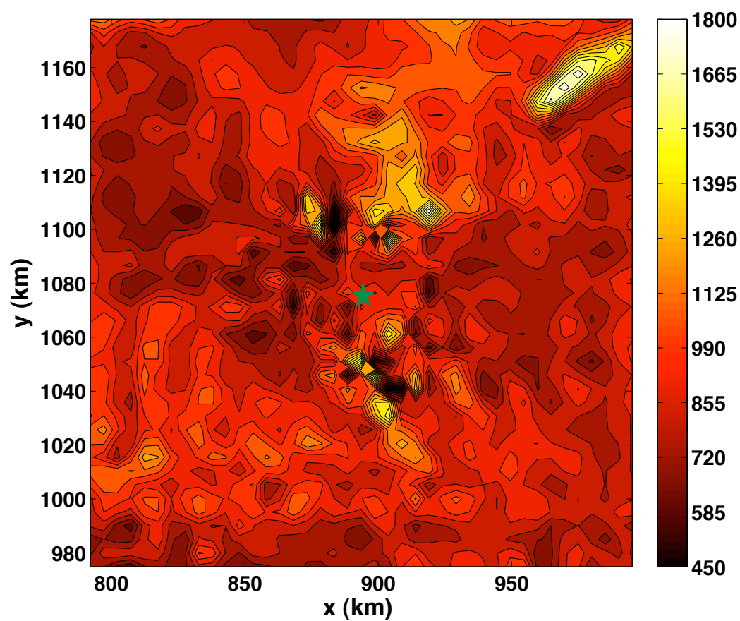
Figure 6.26: Age (ka) at the ice base obtained with steady-state anisotropic simulation. The star indicates the location of the Dome Fuji ice core drilling site.
