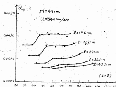
Fig. 17 Local heat transfer coefficient \alpha_l as function of x + l .
