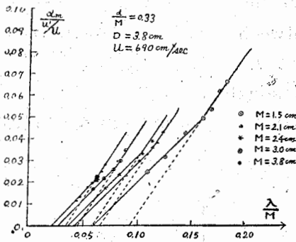
Fig. 5 Relation between a_m/(u'/U) and \lambda/M for various values of M ,
