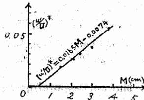
Fig. 4 Relation between mesh length M and intensity of turbulence which corresponds to the minimum points of curves in Fig. 3, (u'/U)^* .
