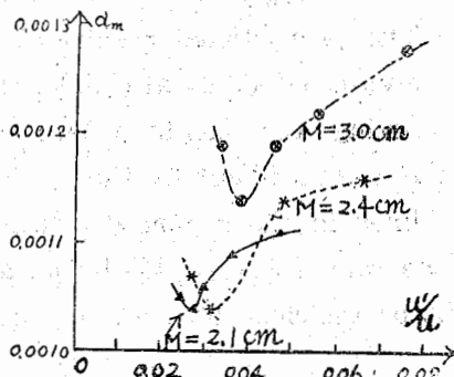
Fig. 3 Mean heat transfer coefficient a_m as function of intensity of turbulence u'/U .
