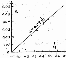
Fig. 6 Ordinate ( a ) represents the values of \lambda/M where \lambda/M -axis is cut by straight lines which lie in the region smaller than the inflection points in Fig. 5.
