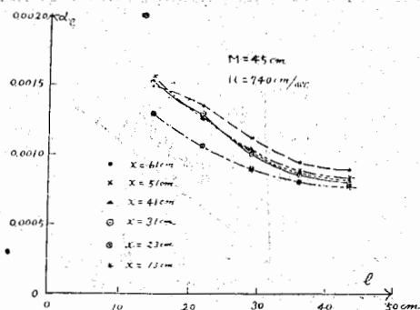
Fig. 16 Local heat transfer coefficient \alpha_l as function of l .
