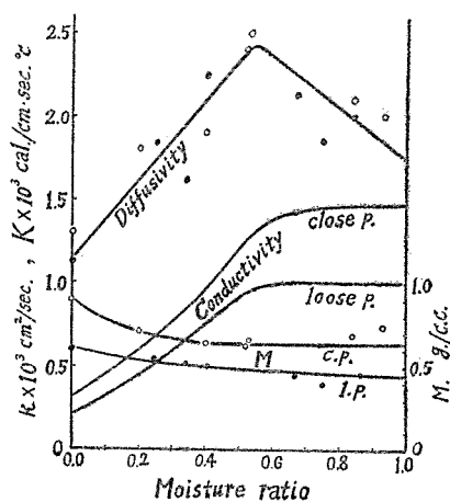
Fig. 6. Thermal diffusivity, conductivity and dried soil mass per unit volume of wet soil with respect to the moisture ratio.
