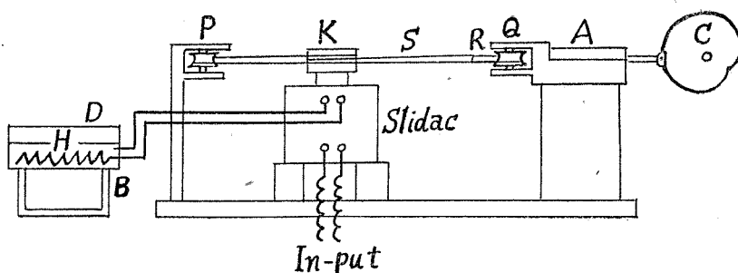
Fig. 3. Apparatus for measuring the thermal diffusivity.
