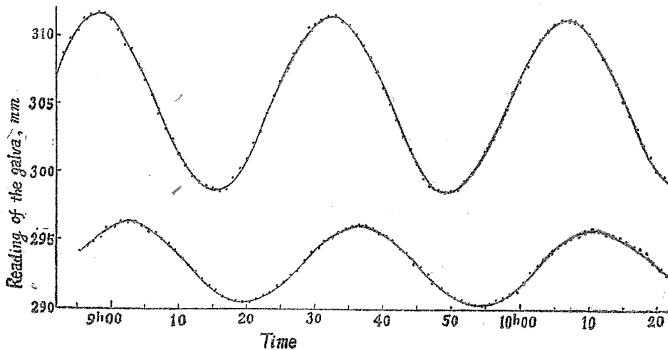
Fig. 5. Temperature-time curves of the experiment No. 15.
