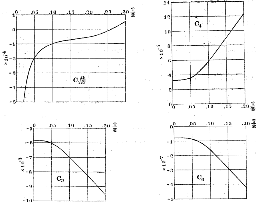
Fig. 1. c_1 , c_2 , c_4 and c_6 in the 7 or 8 terms approximation as functions of T/\theta .
