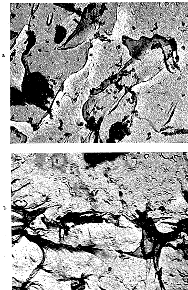
Fig. 4. a: 560°C tempered eutectoid steel. b: 500°C tempered eutectoid steel. \times 40,000
