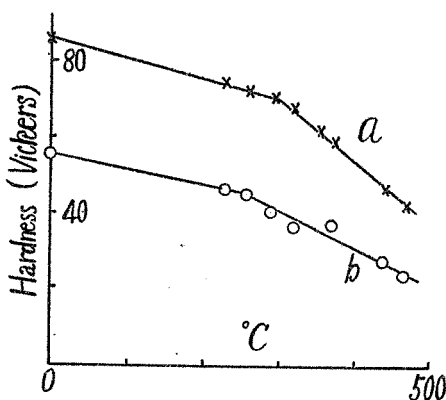
Fig. 2. Variation with temperature of Vicker's hardness of steel.
