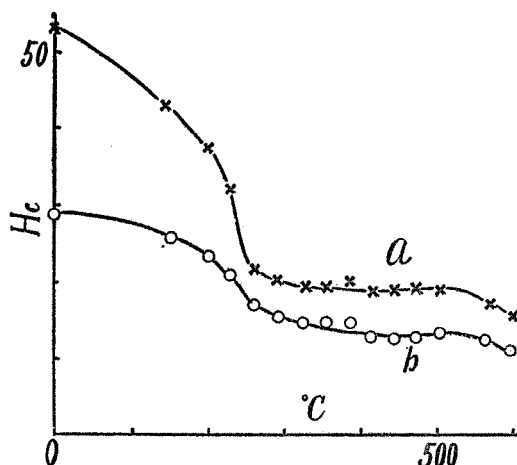
Fig. 1. Variation with temperature of coercive forces of steels.
