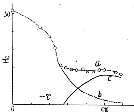
Fig. 5. a: measured curve. b: the curve of coercive force due to internal stress. c: the curve of coercive force due to precipitation of cementite.
