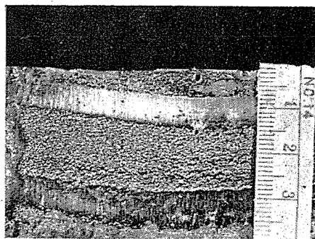
No. 4 Ice filaments layer Soil A. Exp. No. 68 r = 2.77 M = 0.23
