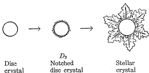
Fig. 2. Growth of disc crystal
