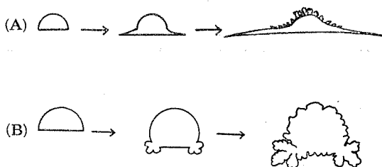
Fig. 3. Two types of growth of semicircular disc crystal
