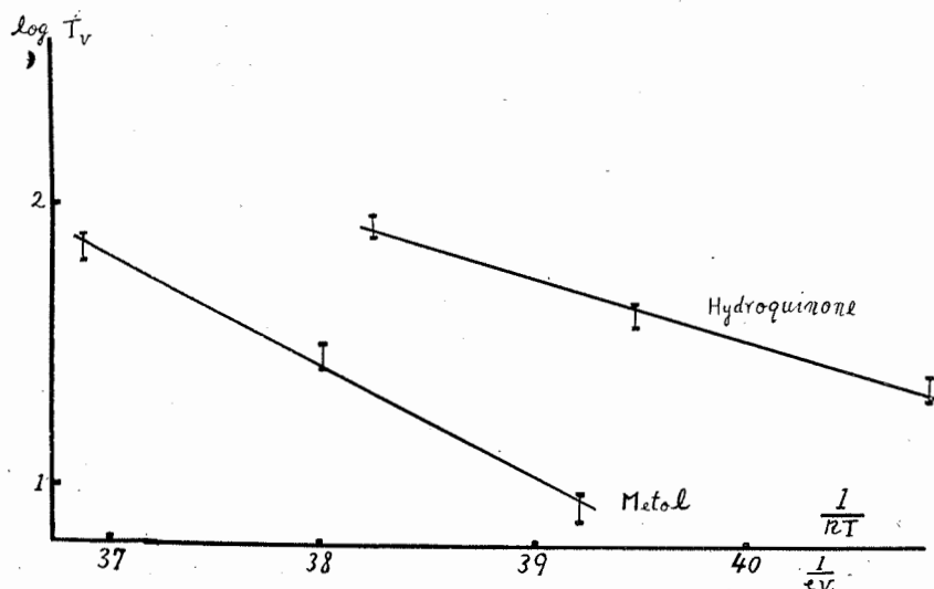
Fig. 3. The relation between the induction periods and the temperature using metol and hydroquinone developer and plate in which silver iodide is contained by 40 Mol %.
