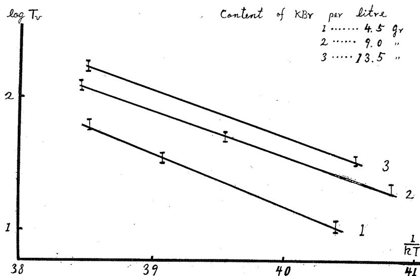
Fig. 2. The relation between the induction periods and temperatures using metol developers, in which KBr is contained in various proportions, and pure silver bromide emulsions.
