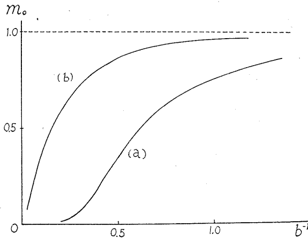
Fig. 3. m_0 as functions of b^{-1} .
