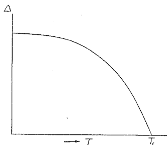
Fig. 1. Temperature variation of \Delta .
