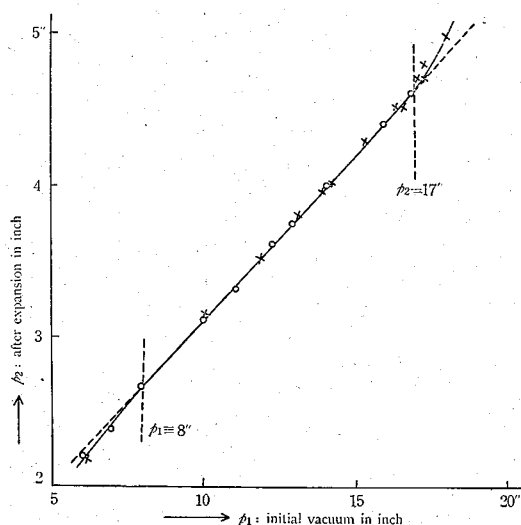
Fig. 1. The relation between p_1 and p_2 ; p_0 = 20.1'' .
