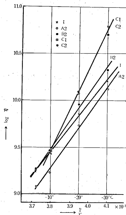
Fig. 50. Calculation of the activation energy.
