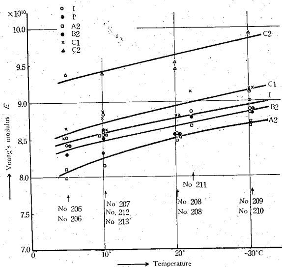
Fig. 37. The relation between YOUNG's modulus and temperature.
