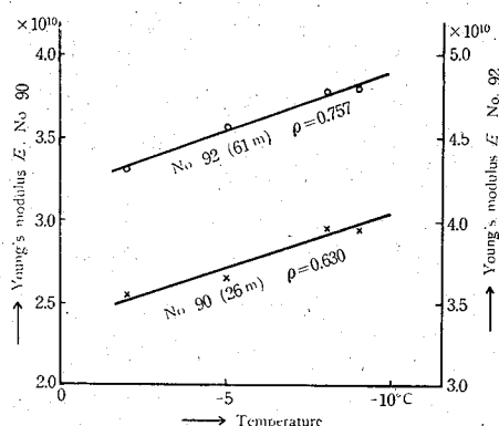
Fig. 28. Temperature dependency of YOUNG's modulus; 1957 core.
