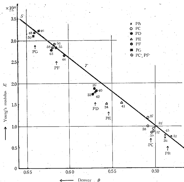
Fig. 12. YOUNG's modulus versus density; samples of deep pit, PC' and PF' are two years old.
