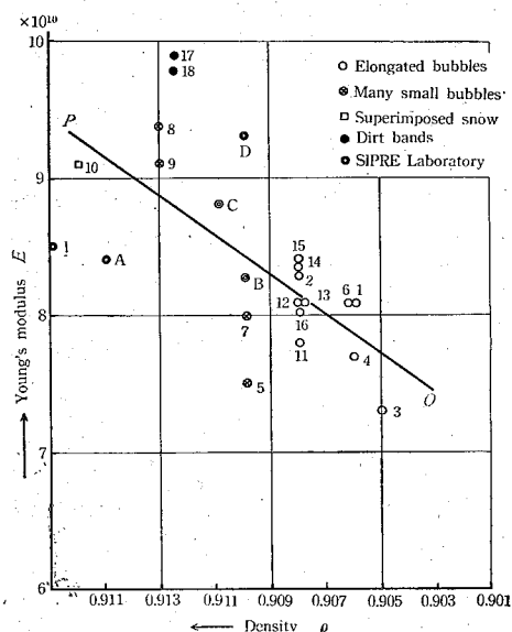
Fig. 7. YOUNG's modulus versus density; tunnel ice.
