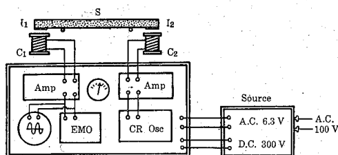
Fig. 2. The schematical diagram of the portable visco-elastic meter.
