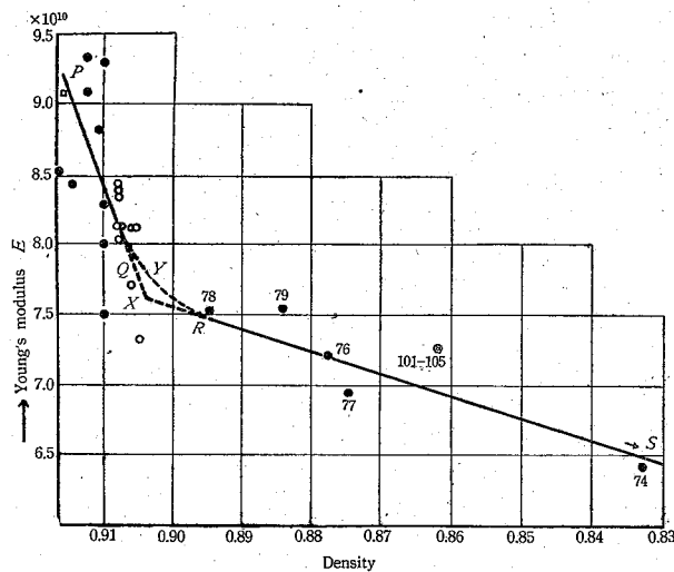
Fig. 17. YOUNG's modulus versus density; tunnel ice and core samples.
