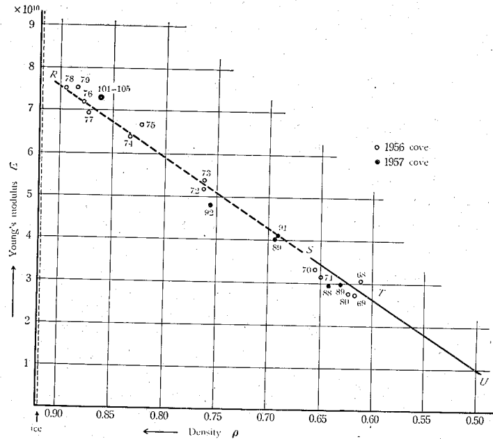
Fig. 16. YOUNG's modulus versus density; 1956 core and 1957 core.
