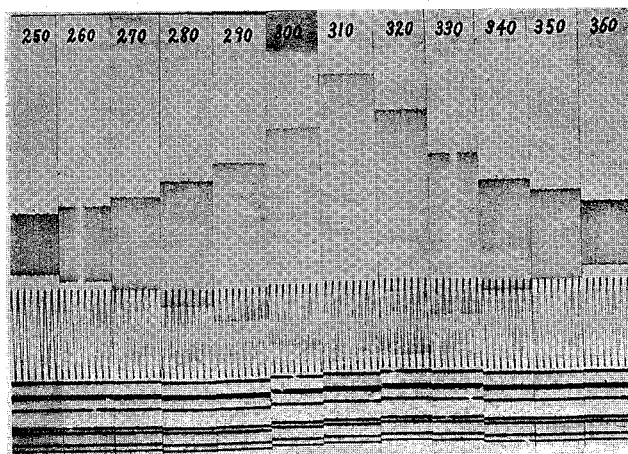
Fig. 33. 1957 core, 26 m; No. 90, \rho=0.630 , E=2.96 \times 10^{10} , \tan \delta=0.074 .
