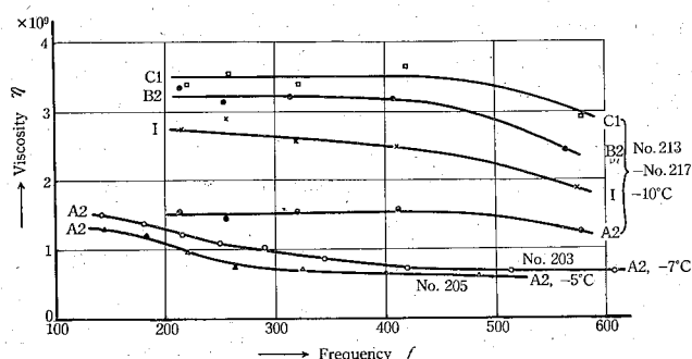
Fig. 52. Frequency dependency of viscosity; MAXWELL model, Nos. 203, 205, 213-217.
