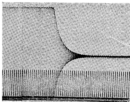
Fig. 41. C2 ice, No. 207, -10^{\circ}\text{C} , \rho=0.910 , E=9.39 \times 10^{10} , \tan \delta=0.0206 .
