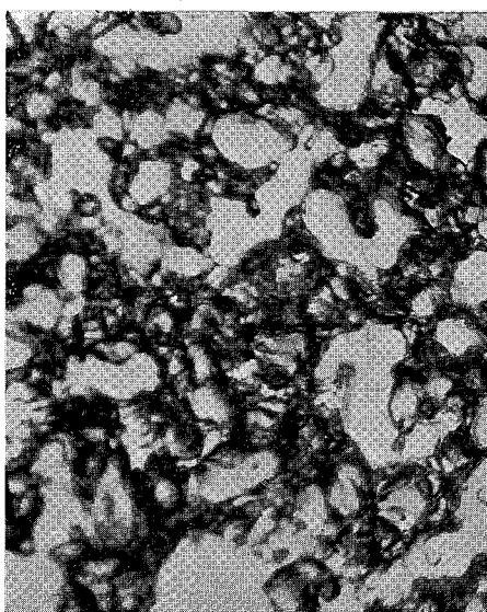
Fig. 8. Deep pit PB, \rho = 0.49 , \times 10.5 .
