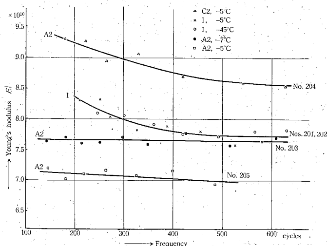
Fig. 39. Frequency dependency of YOUNG'S modulus; -4.5^{\circ}\text{C} - -7^{\circ}\text{C} , Nos. 201-205.
