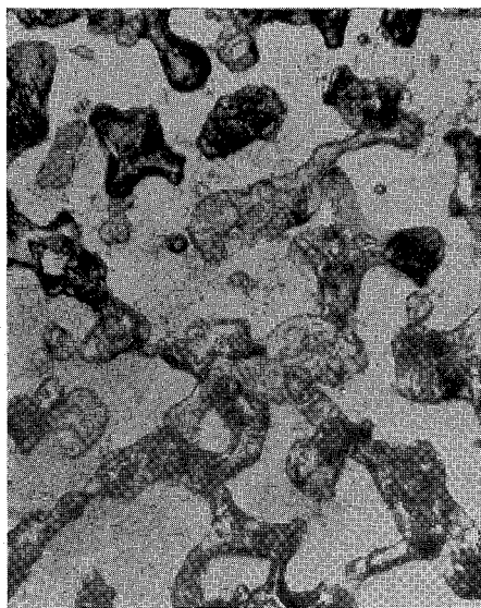
Fig. 11. Deep pit PG, \rho = 0.64 , \times 10.5 .
