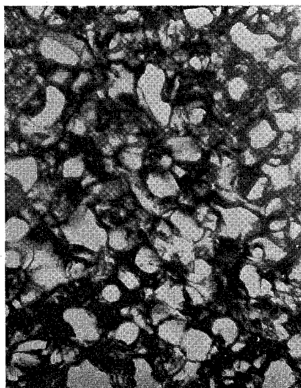
Fig. 9. Deep pit PD, \rho = 0.57 , \times 10.5 .
