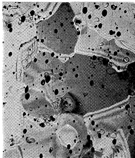
Fig. 6. C2 ice, 680' from the entrance of the tunnel; \rho = 0.910 , \times 7.5 .
