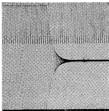
Fig. 29. Tunnel ice No. T2, \rho=0.908 , f=254 , E=8.3 \times 10^{10} , \tan \delta= 0.0332 , -5^{\circ}\text{C} .
