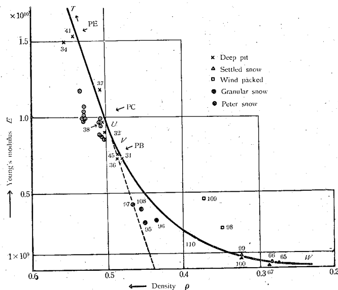
Fig. 23. YOUNG's modulus versus density; snow near the surface of ice cap.
