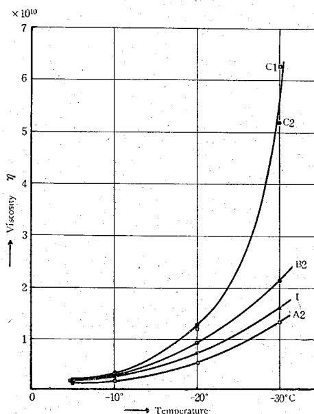
Fig. 49. Temperature dependency of viscosity; MAXWELL model, Nos. 206-212.
