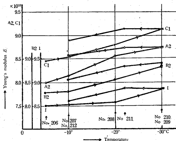
Fig. 36. Hysteresis phenomenon in the relation between YOUNG's modulus and temperature; Nos. 206'-212.
