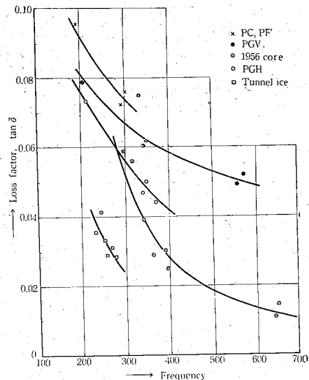
Fig. 35. The frequency dependency of loss factor.
