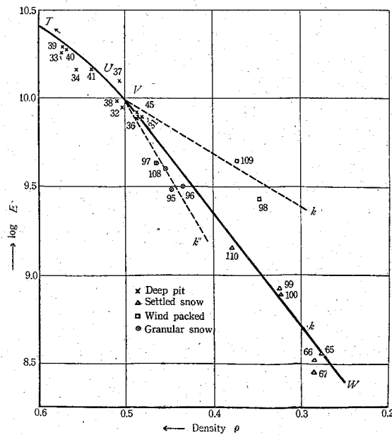
Fig. 24. \log E-\rho curve; snow near the surface of ice cap.
