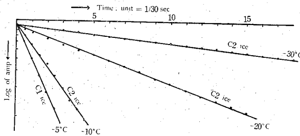
Fig. 1. The mode of damping at various temperatures.
