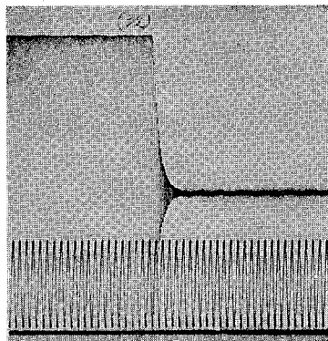
Fig. 32. 1957 core, No. 92, 61 m, \rho= 0.757 , f=360 , E=4.78 \times 10^{10} , \tan \delta=0.049 , -9^{\circ}\text{C} .
