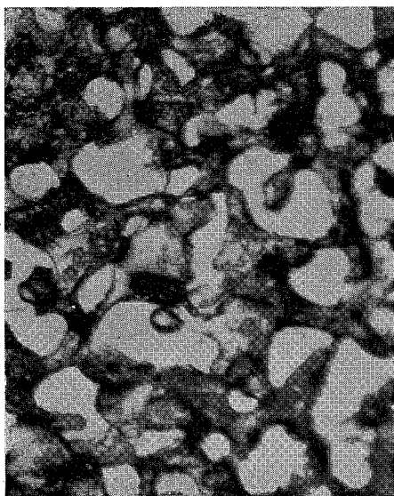
Fig. 10. Deep pit PF, \rho = 0.61 , \times 10.5 .
