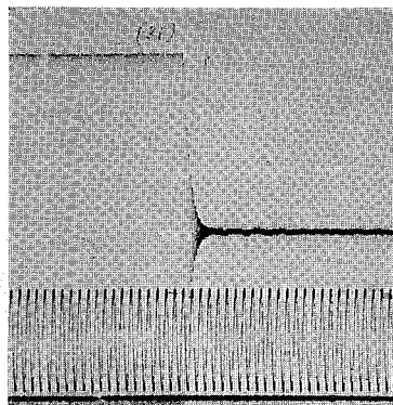
Fig. 31. Coarse grain snow, No. 41. \rho=0.538 , f=281 , E=1.53 \times 10^{10} , \tan \delta=0.0905 , -9^{\circ}\text{C} .
