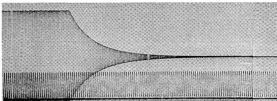
Fig. 46. B2 ice, No. 208, -20^{\circ}\text{C} , \rho = 0.910 , E = 8.79 \times 10^{10} , \tan \delta = 0.0054 .
