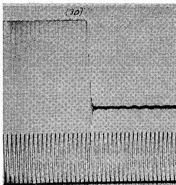
Fig. 30. New soft snow, No. 67, \rho=0.288 , f=105 , E=0.028 \times 10^{10} , \tan \delta=0.361 , -9^{\circ}\text{C} .
