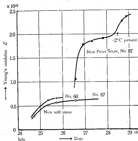
Fig. 27. Age hardening of soft snow and Peter snow.
