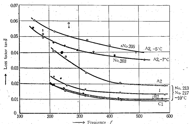
Fig. 51. Frequency dependency of \tan \delta ; Nos. 203, 205, 213-217.
