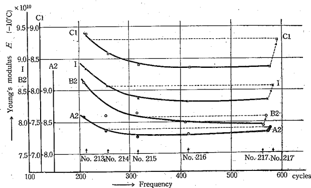
Fig. 38. Frequency dependency of YOUNG's modulus; -10^{\circ}\text{C} , Nos. 213-217'.
