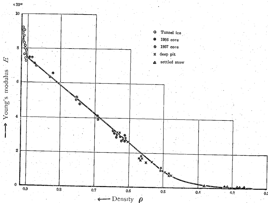
Fig. 25. The relation between YOUNG's modulus and density for the whole range of Greenland ice and snow.
