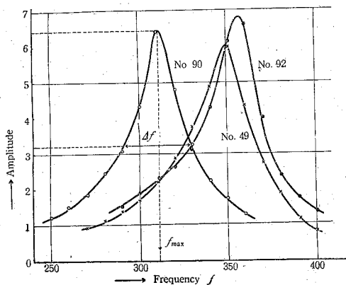
Fig. 34. The resonance curve; amplitude versus frequency.
