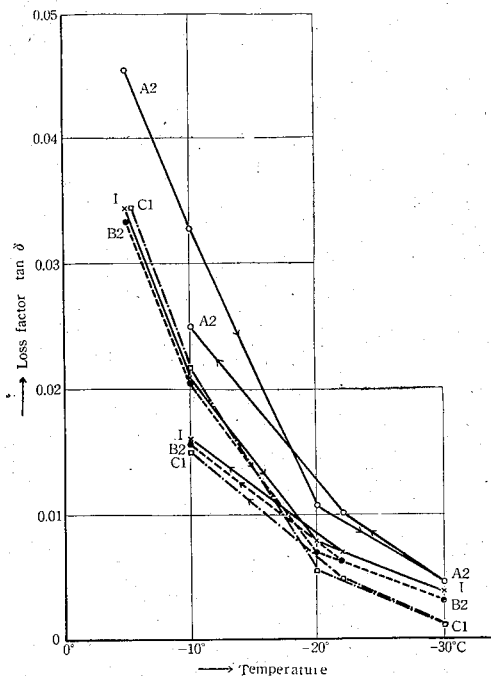
Fig. 48. Hysteresis phenomenon in the relation between loss factor and temperature.
