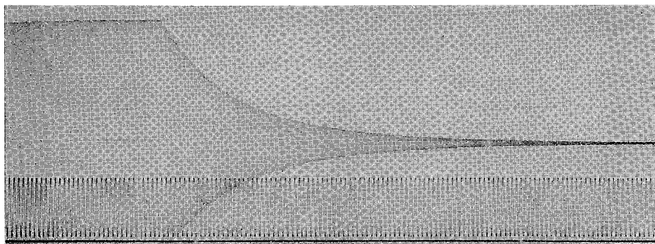
Fig. 47. C1 ice, No. 208, -20^{\circ}\text{C} , \rho = 0.911 , E = 8.79 \times 10^{10} , \tan \delta = 0.0054 .
