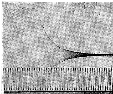
Fig. 45. A2 ice, No. 208, -20^{\circ}\text{C} . \rho = 0.915 , E = 8.55 \times 10^{10} , \tan \delta = 0.0106 .
