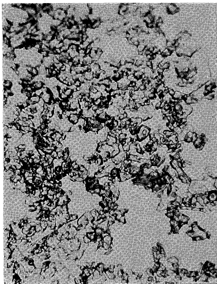
Fig. 20. Wind packed snow, \rho = 0.35 , \times 10.5 .
