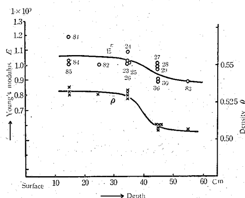
Fig. 22. Vertical distribution of E and \rho in Peter snow of one year old; Sample Nos. 23-30, 81-86.
