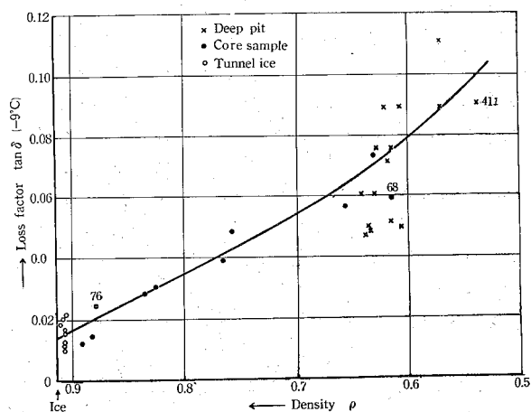
Fig. 53. The relation between loss factor and density.
