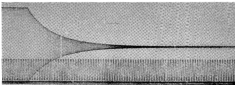
Fig. 42. C2 ice, No. 208, -20^{\circ}\text{C} , \rho=0.910 , E=9.52 \times 10^{10} , \tan \delta=0.0049 .
