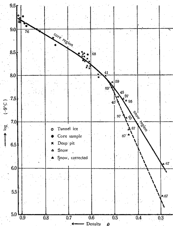
Fig. 54. The relation between viscosity and density; -9^{\circ}\text{C} , frequency between 200-400 cycles.
