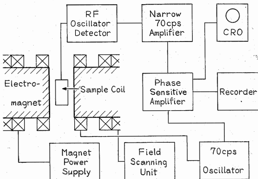
Fig. 2. Block diagram of the NMR spectrometer.
