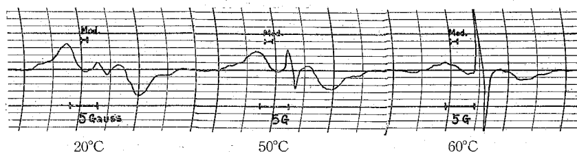
Fig. 5. The proton resonance line derivatives of the sodium iodide dihydrate at 20°, 50°, and 60°C.
