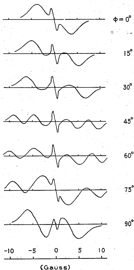
Fig. 3. The dependence of the proton resonance line derivatives of \text{NaBr}\cdot 2\text{H}_2\text{O} on the angle \phi between b -axis and the applied magnetic field H_0 in a - b plane.
