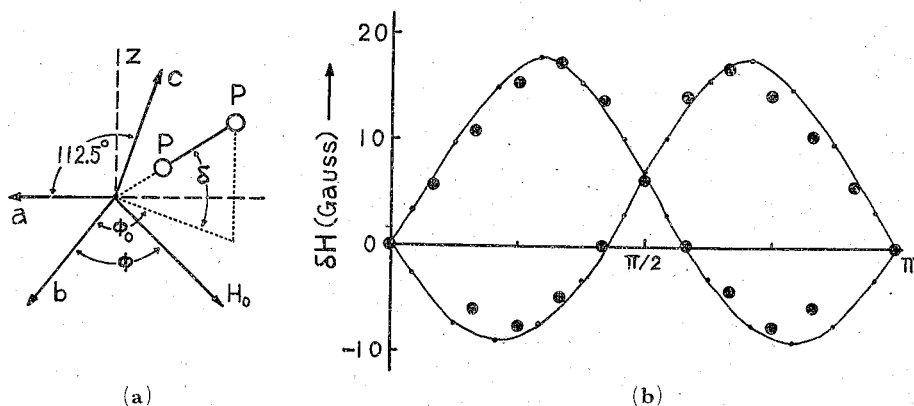
Fig. 4. (a) Diagram of the relations of the applied field H_0 and the proton-proton line to crystal axes of the sodium bromide dihydrate. (b) PAKE curves for \text{NaBr} \cdot \text{H}_2\text{O} rotated about the z -axis. Solid curves are the plots of the theoretical value for \phi_0 = \pm 52^\circ , \delta = \pm 20.5^\circ , and 2\alpha = 10.5 gauss.
