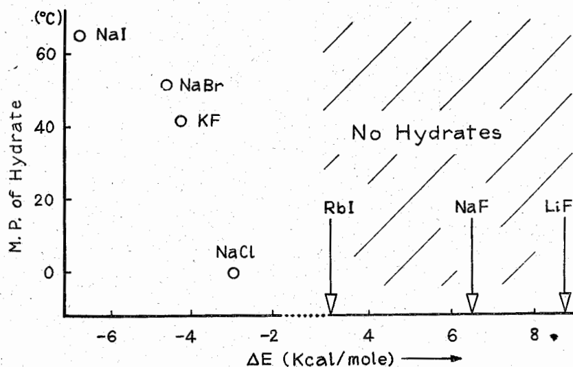
Fig. 1. Electrostatic energy difference \Delta E between (\text{M} \cdot \text{X}) and (\text{M} \cdot \text{OH}_2 \cdot \text{X}) versus melting point of the actual hydrate. \Delta E of the alkali halide which has no hydrate is represented by the arrow.
