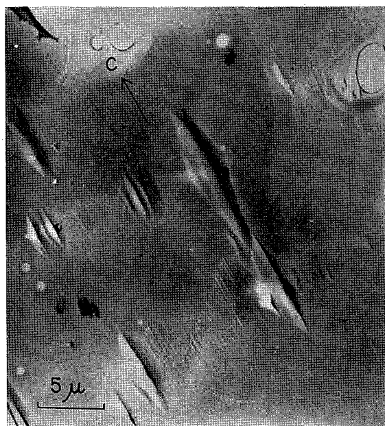
Fig. 3. Elongated spindle shape of etch pits on a prism plane caused by deformation of ice crystal. Notice that dislocations pile up on the basal plane. Electron photomicrograph.
