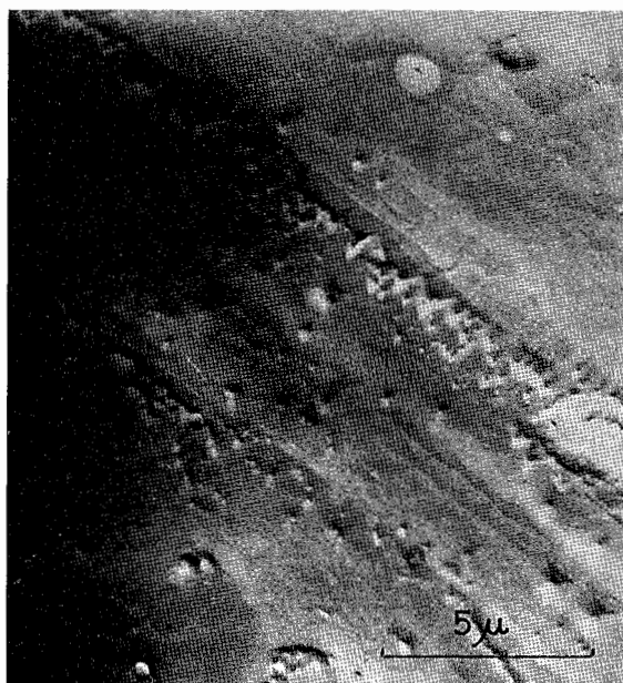
Fig. 8. Well developed trigonal etch pits along a slip band. Electron photomicrograph.
