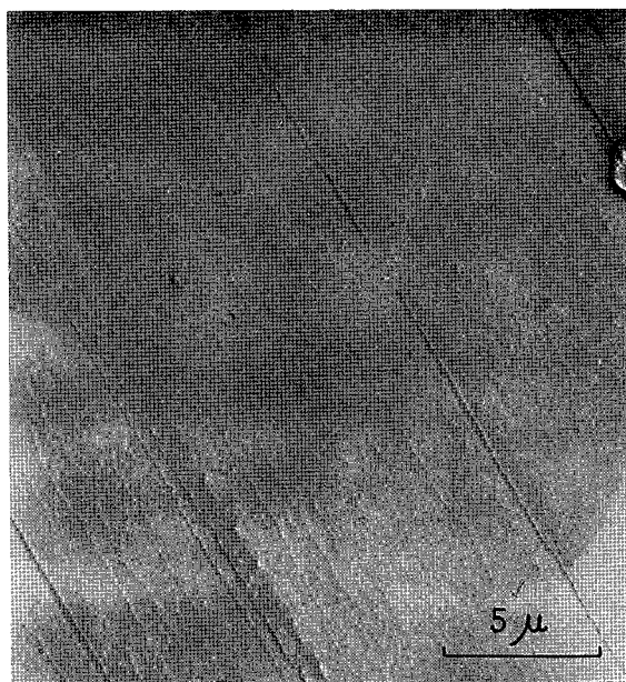
Fig. 7. Slip lines appeared on a plane making 45 degrees to the basal plane, as a result of tension in a direction perpendicular to the observed surface. Electron photomicrograph of not well developed etch pits. Notice slip bands separated about 10\ \mu among which many micro-slip lines are visible.
