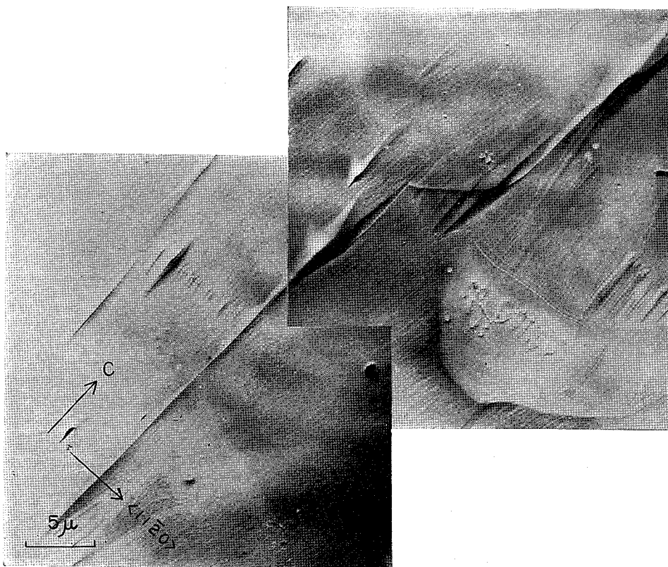
Fig. 5. Arrangement of etch pits on a prism plane along a small angle boundary. Notice a row of elongated etch pits in center is shifting and also the pile up of dislocations on the basal plane. Electron photomicrograph.
