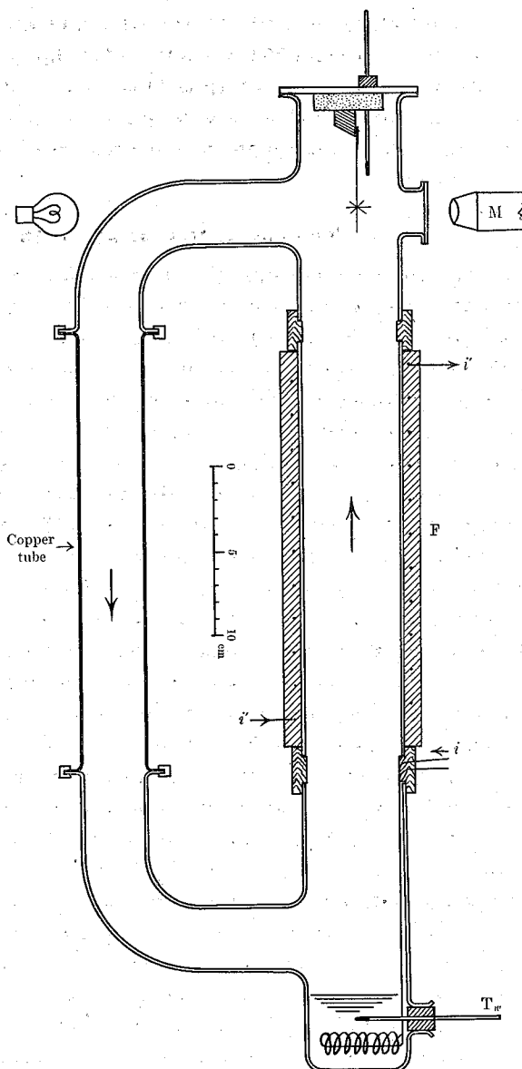
Fig. 4. Apparatus No. 4.
