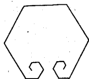
a) Horizontal section of a crevasse hoar, after Seligman.
