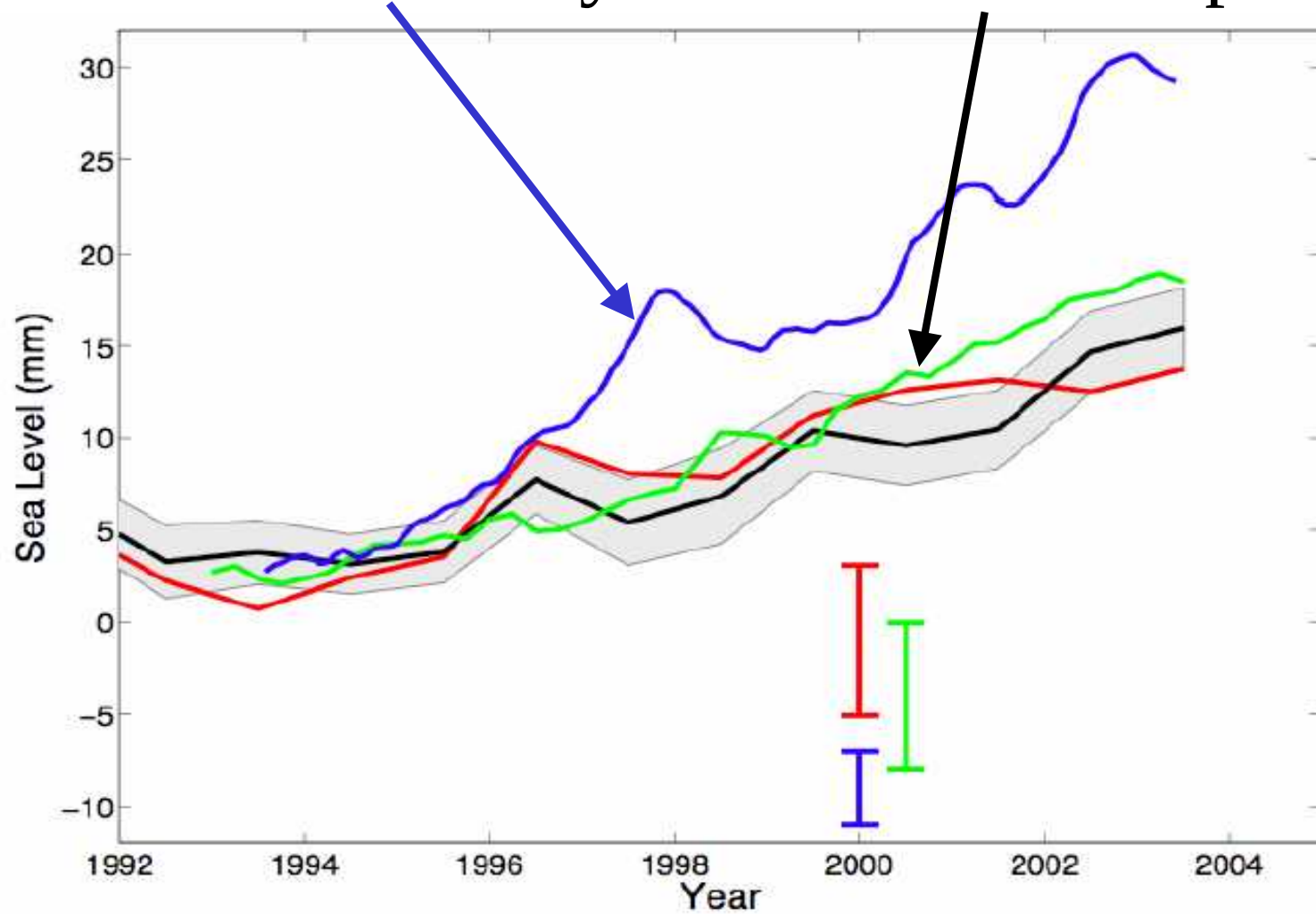
Figure 5.5.7. Thermal expansion curves for 1993–2003, average over 60°S–60°N, based on Levitus et al. (2005a) temperature data (in black; 0–700 m layer), Ishii et al. (2006) (in red; 0–700 m layer) and Willis et al. (2004) (in green; 0–750 m layer). Shaded area and vertical red and green bars represent the 95% errors of the black, red and green curves respectively. The blue curve is the observed global mean sea level by satellite altimetry (yearly-mean, averaged over 65°S–65°N).
