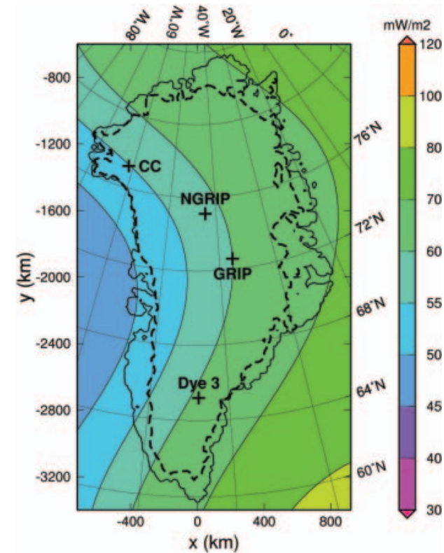
Fig. 3. Distribution of the geothermal heat flux by Pollack and others (1993) scaled to a value of 60 mW m −2 at GRIP (for simulation hf_psc). The heavy dashed line indicates the present-day ice margin.
