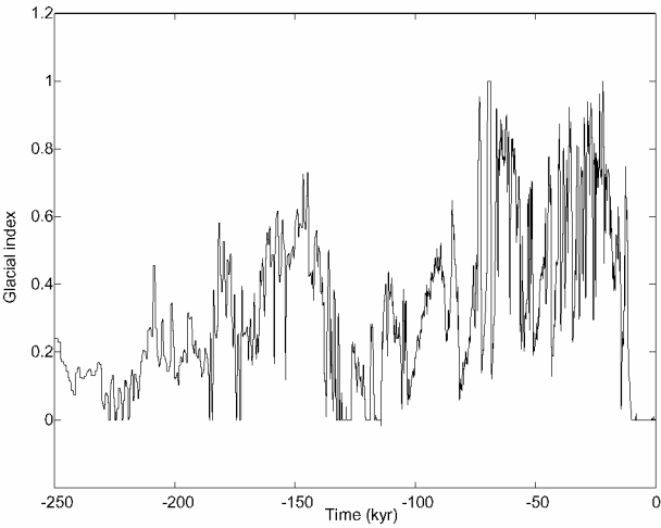
Fig. 2. Glacial index g(t) as a function of time. This index scales the GRIP \delta^{18}\text{O} record (Dansgaard and others, 1993) to represent glacial ( g = 1 ) and present ( g = 0 ) conditions.
