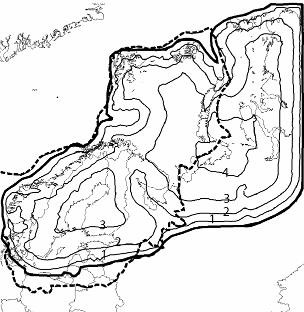
Fig. 3. The simulated ice-sheet extent (thick solid line) and thickness (solid contours, spacing 1 km) at the LGM (20 kyr BP). The thick dashed line indicates the LGM ice-sheet extent by QUEEN (Svendsen and others, 1999; Thiede and others, 2001).
