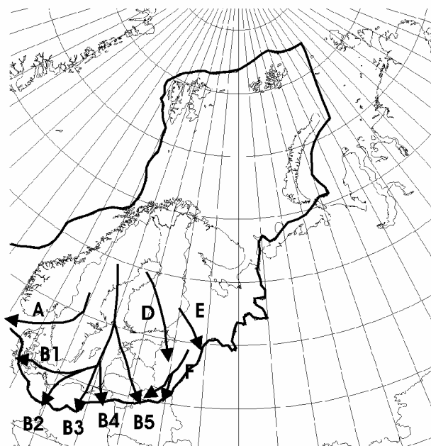
Fig. 1. Ice-sheet extent at LGM (solid line) according to QUEEN (Svendsen and others, 1999; Thiede and others, 2001). Added to this are the approximate positions for the ice streams identified by Boulton and others (2001): the Norwegian Channel ice stream (A), the Baltic Ice Stream (B), the Danish sub-lobe (B1), the Oder sub-lobe (B2), the Wisla sub-lobe (B3), the Kurshkiy sub-lobe (B4), the Riga sub-lobe (B5), the Finnish ice stream (D), the Karelian ice stream (E) and the Novgorod ice stream (F).
