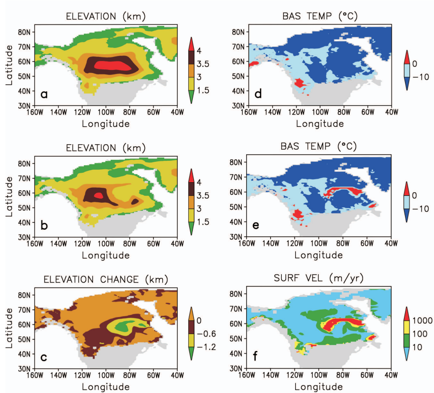
Figure 3: Heinrich event VI (in Figure 1) is shown here. Elevation of the LIS (a) before and (b) after that HE. (c) Difference between the elevations before and after the same HE. Basal temperature corrected for pressure melting (d) before and (e) during that HE. (f) Ice-surface velocity during the same HE.
