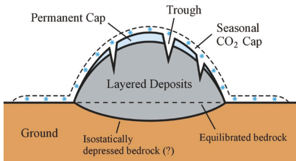
Figure 1: Schematic representation of the seasonal cap, permanent cap and underlying layered deposits for the north polar region of Mars. In the south polar region, the situation is essentially the same; however, the areal extent of the permanent cap is much smaller than that of the layered deposits. The vertical scale is exaggerated by about a factor 150 for the layered deposits, by an unknown factor for the permanent cap and by about a factor 50000 for the seasonal cap.
