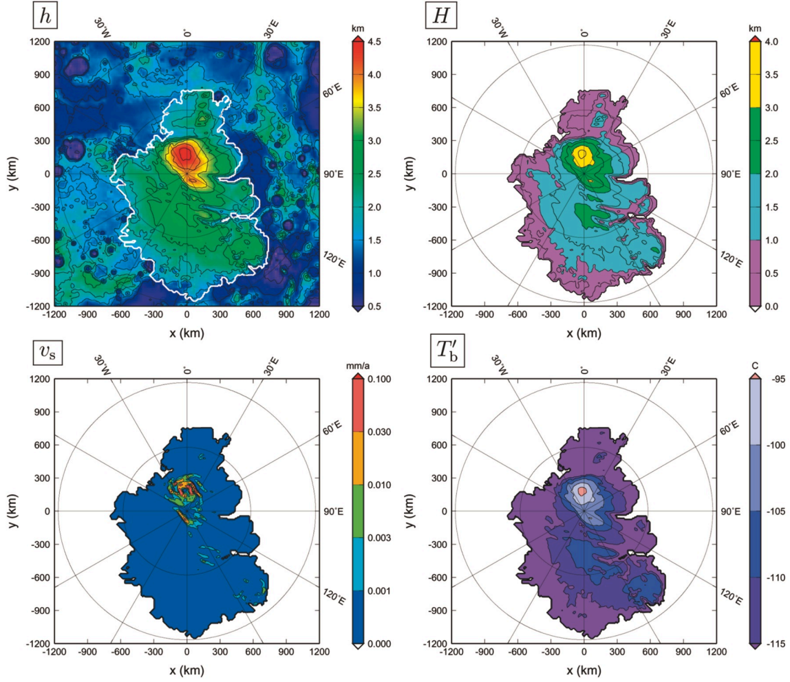
Figure 6: SPLD of Mars: MOLA surface topography h (Smith et al. 1999), computed ice thickness H , computed surface velocity v_s and computed basal temperature T'_b (relative to pressure melting) for present-day steady-state conditions. The thick white line in the surface topography plot indicates the ice margin.
