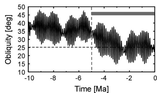
Figure 3: Martian obliquity for the last 10 Ma (Laskar et al. 2004). The grey bar indicates the most recent 5-Ma period with relatively low average obliquity, which favours the formation of polar deposits.
