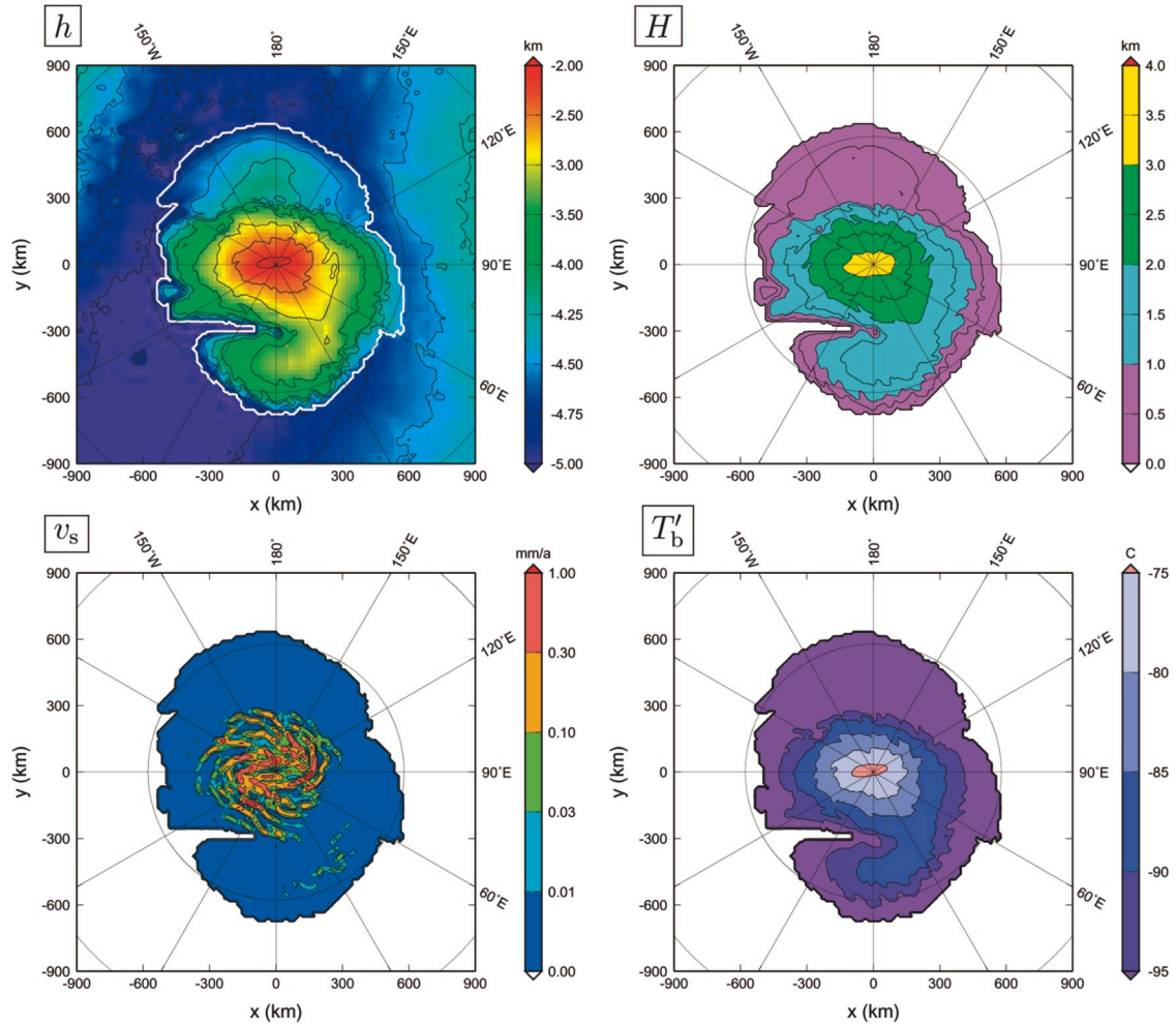
Figure 5: NPLD of Mars: MOLA surface topography h (Smith et al. 1999), computed ice thickness H , computed surface velocity v_s and computed basal temperature T'_b (relative to pressure melting) for present-day steady-state conditions. The thick white line in the surface topography plot indicates the ice margin.
