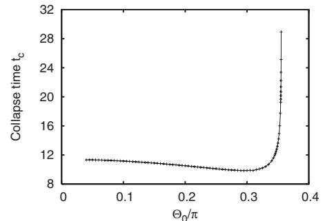
FIG. 10. Time of the triple 234 collapse, t_c , versus \Theta_0 .
