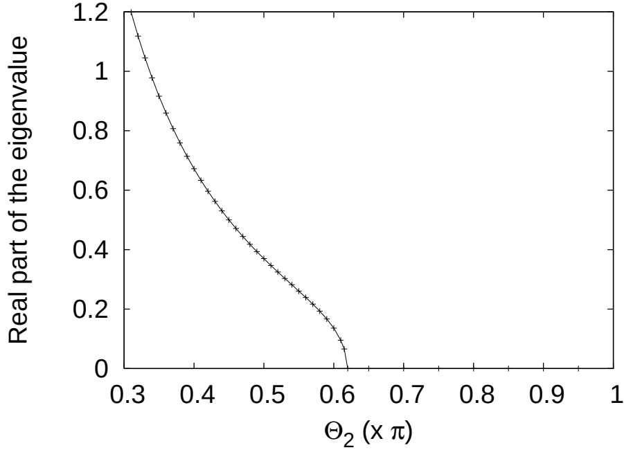
Figure B1: Maximum real part among the eigenvalues \lambda^+ of the linearized matrix \mathcal{S}^+ for \Theta_2 \in (\Theta_1, \pi) with \Theta_1 = 0.3\pi .
