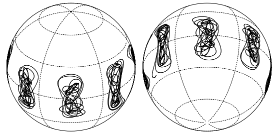
FIG. 5: Chaotic motion of the eight point vortices in the full system (1).
