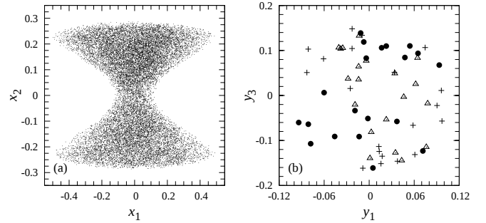
FIG. 3: Orbit of the Poincaré map: (a) Its projections onto the \mathbf{x} -plane; (b) onto the (y_1, y_3) -plane when it enters in a neighborhood of \mathcal{M} . In plate (b), ‘+’ represents for 1st-20th visits, ‘•’ for 21st-40th, and ‘Δ’ for 41st-60th.
