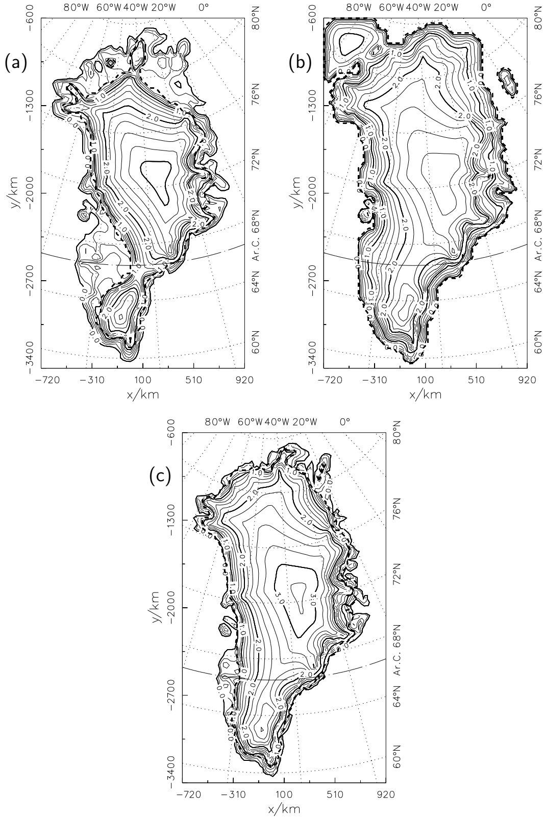
Figure 5: Simulation gp9: surface topography for t = -127 kyr (Eemian Ice Volume Minimum, plot a), t = -21 kyr (Last Glacial Maximum, plot b) and t = 0 (present, plot c), in km a.s.l. The spacing between the isolines is 200 m. The dashed heavy line indicates the ice margin.
