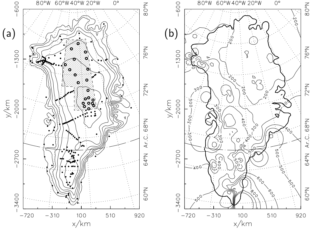
Figure 3: Left (plot a): positions of accumulation measurements listed by Ohmura and Reeh (1991) (small dots) and by Bolzan and Strobel (1994) and Wilhelms (1996) (open circles), on which our new accumulation map, used for simulations gp6 – gp9, is based. The shaded area indicates the region where the data of Ohmura and Reeh are blanked out. Right (plot b): new accumulation map; accumulation rate in mm WE per year (spacing 100 mm WE per year).
