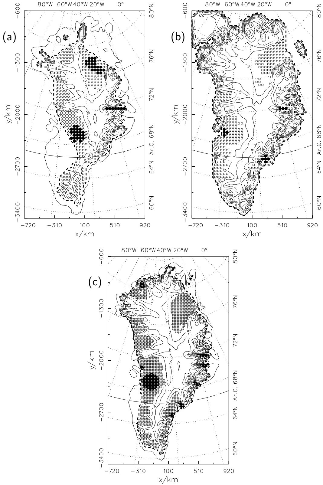
Figure 6: Simulation gp9: homologous temperature at the ice base (in ^{\circ}\text{C} ), for t = -127 kyr (Eemian Ice Volume Minimum, plot a), t = -21 kyr (Last Glacial Maximum, plot b) and t = 0 (present, plot c). The spacing between the isolines is 3^{\circ}\text{C} . Open circles (full circles) indicate positions where the basal ice is at the pressure melting point with no temperate layer above (with a temperate layer above). The dashed heavy line indicates the ice margin.
