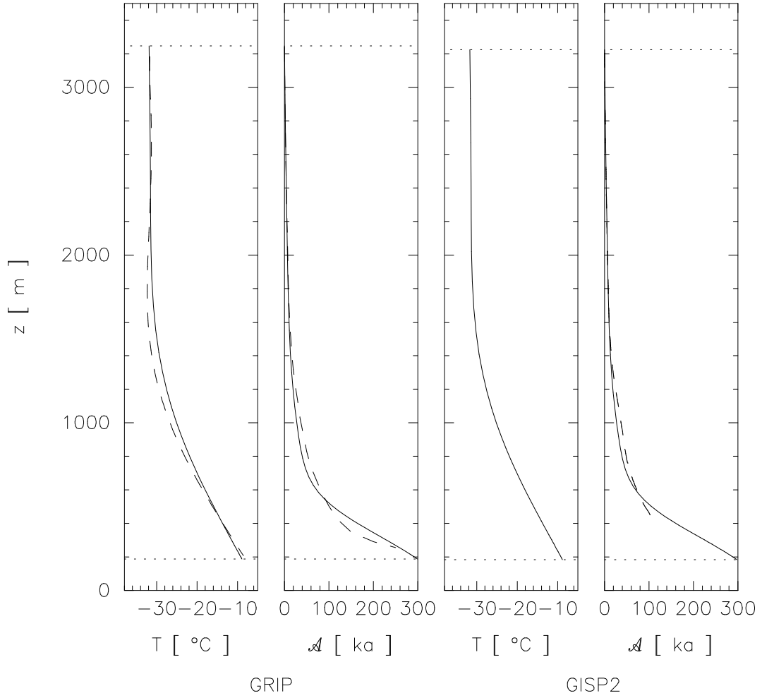
Figure 9: Simulation gp9: present temperature and age profiles for GRIP and GISP2. a) temperature profile for GRIP, together with measured data (by Johnsen et al. (1995); dashed). b) age profile for GRIP, together with the dating by Dansgaard et al. (1993) (dashed). c) temperature profile for GISP2, together with measured data (by Cuffey et al. (1995); dashed). d) age profile for GISP2, together with the dating by Meese et al. (1994), Sowers et al. (1993) (dashed).
