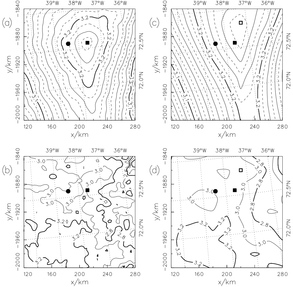
Figure 8: The present vicinity of Summit. Left: measured surface topography (plot a) and ice thickness (plot b), by Hodge et al. (1990). Right: simulated surface topography (plot c) and ice thickness (plot d) from simulation gp9. Full squares show the GRIP position (actual summit), full circles the GISP2 position and open squares the position of the simulated summit (only in panels c, d). Surface elevations are given in km a.s.l. (spacing 10 m), ice thicknesses in km (spacing 200 m).
