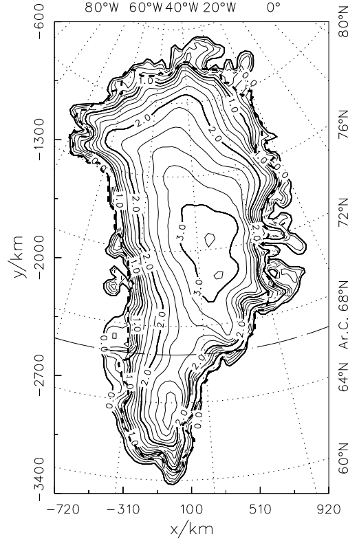
Figure 1: Measured surface topography h^{\text{today}} of the present Greenland Ice Sheet, according to Letréguilly et al. (1991) for the whole of Greenland, and Hodge et al. (1990) for the Summit region (in km a.s.l.). The spacing between the isolines is 200 m. The dashed heavy line indicates the ice margin.
