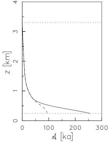
Figure 2: Computed age-depth profiles of the present Greenland Ice Sheet, for the column (x, y) = (200 \text{ km}, -1880 \text{ km}) situated nearest to the actual GRIP position. Solid: simulation gp5, with the improved basal boundary condition (23). Dashed: simulation gp4, still with the old boundary condition (22).
