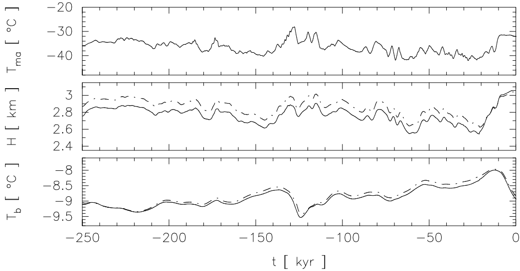
Figure 7: Simulation gp9: time evolution of the mean annual air temperature T_{\text{ma}} at GRIP (deduced from the surface temperature forcing, Eq. (9)), the ice thicknesses H at GRIP (solid) and GISP2 (chain-dotted), and the basal temperatures T_{\text{b}} at GRIP (solid) and GISP2 (chain-dotted).
