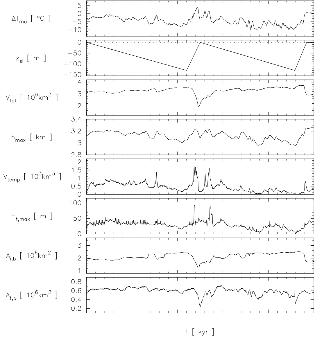
Figure 4: Simulation gp9: model forcings \Delta T_{\text{ma}} , z_{\text{sl}} ; time evolution of V_{\text{tot}} , h_{\text{max}} , V_{\text{temp}} , H_{\text{t,max}} , A_{\text{i,b}} and A_{\text{t,b}} (as defined in the main text).
