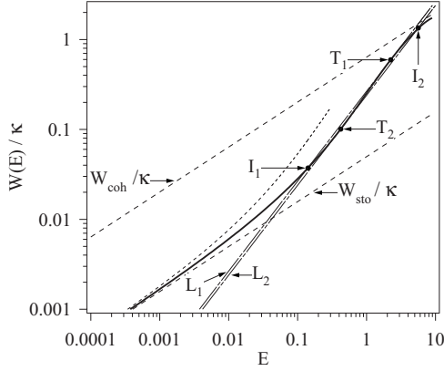
FIG. 4. The log-log plot of \frac{1}{\kappa}W(E) versus E at \omega_G = \omega_0 for U_G^0 = 1 . The dashed lines indicate \frac{1}{\kappa}W_{sto} and \frac{1}{\kappa}W_{coh} , respectively. T_n and I_n ( n=1 and 2 ) indicate the contact points and intersection points between \frac{1}{\kappa}W(E) and the tangent lines L_1 and L_2 (dot-long-dashed lines). The energy at each point is E_{I_1} = 0.14 at I_1 , E_{T_1} = 2.24 at T_1 , E_{I_2} = 5.62 at I_2 , and E_{T_2} = 0.42 at T_2 .
