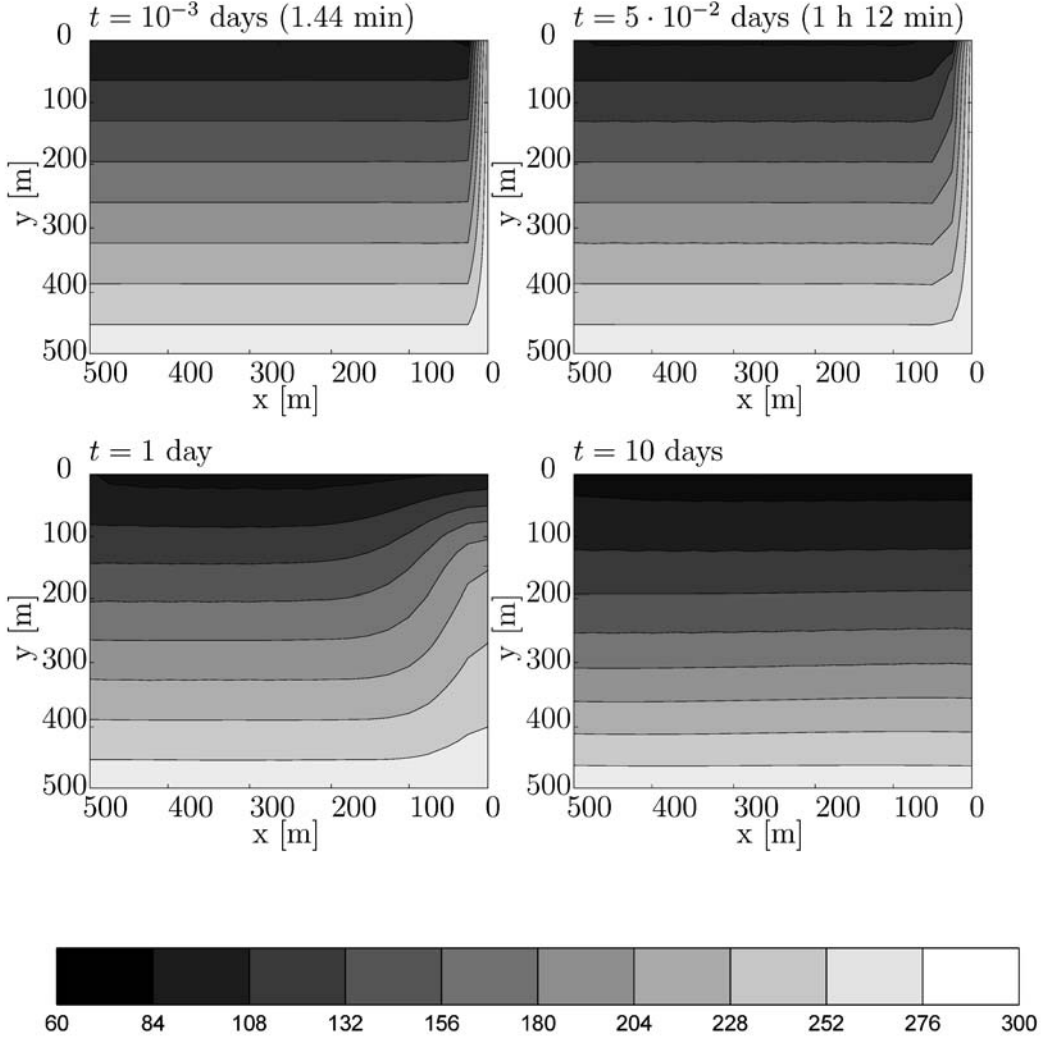
Fig. 7. Case 4 ( f=10^8 ): Evolution of the temperature field (in K) in the 500\text{ m} \times 500\text{ m} area next to the volcanic vent shown in Fig. 3.
