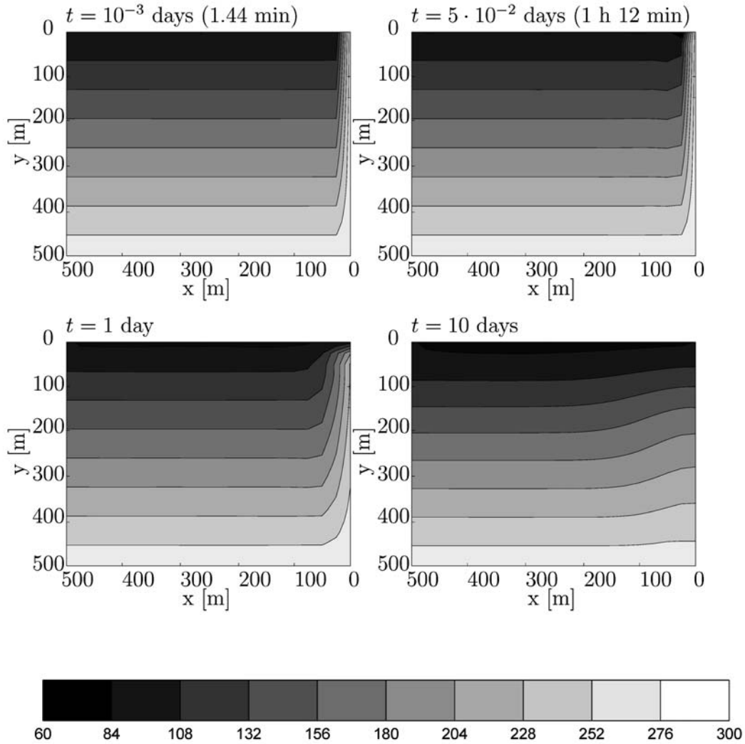
Fig. 6. Case 3 ( f=10^7 ): Evolution of the temperature field (in K) in the 500\text{ m} \times 500\text{ m} area next to the volcanic vent shown in Fig. 3.
