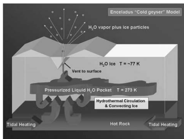
Fig. 2. "Cold geyser model" for cryovolcanism on Enceladus: Pressurized sub-surface water erupts through a volcanic pipe (vent) into the atmosphere. Credit: NASA/JPL/SpaceScience Institute/Cassini-Huygens.
