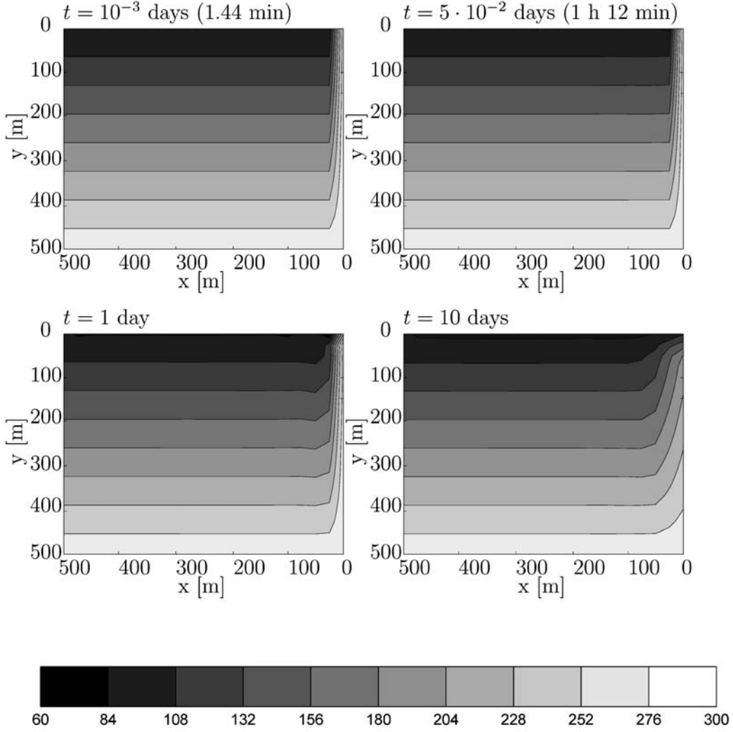
Fig. 5. Case 2 ( f=10^6 ): Evolution of the temperature field (in K) in the 500 m × 500 m area next to the volcanic vent shown in Fig. 3.
