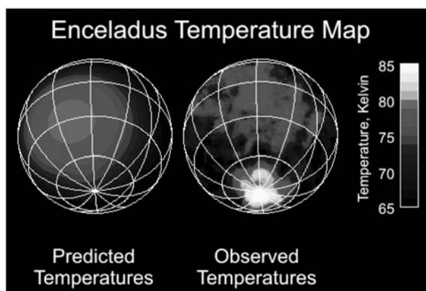
Fig. 1. Predicted (radiation balance) vs. observed (composite infrared spectrometer CIRS onboard the Cassini spacecraft) surface temperatures of Enceladus. The south polar region shows a warm spot due to active cryovolcanism. Credit: NASA/JPL/GSFC.
