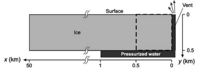
Fig. 3. Set-up of the model cryovolcano. The adjacent ice layer is 50 km long and 500 m thick. The dashed square marks the 500 \text{ m} \times 500 \text{ m} area next to the volcanic vent for which the evolution of the temperature field will be plotted in Figs. 4–7.
