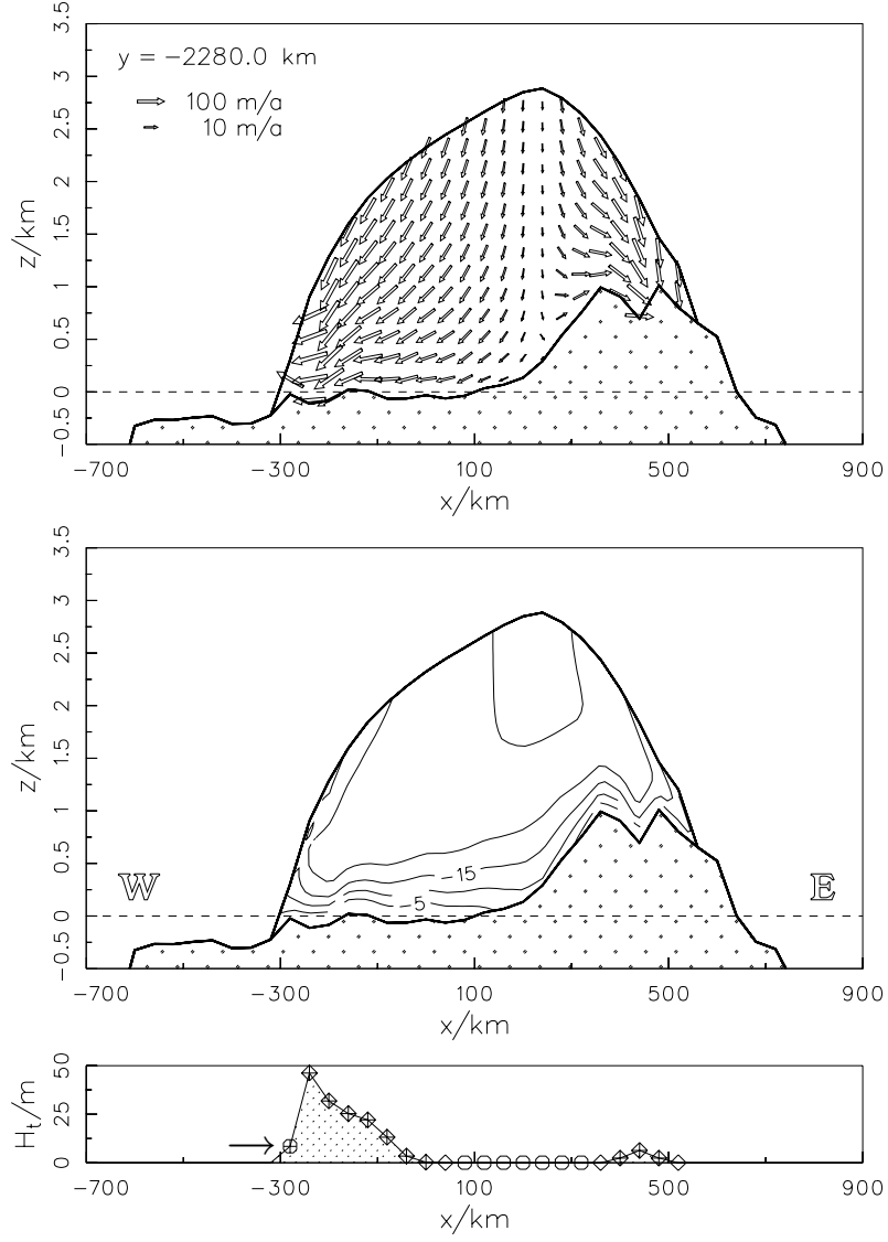
Figure 14: Final state of simulation: Transect at y = -2280 km. Top: ice velocity. Middle: homologous ice temperature (in °C). Bottom: thickness of the basal layer of temperate ice (open circles: cold ice base; open diamonds: temperate ice base with no temperate ice layer above; full diamonds: basal layer of temperate ice with a melting CTS; full circle (see \rightarrow in the plot): basal layer of temperate ice with a freezing CTS).
