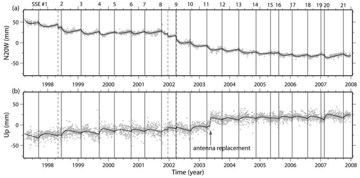
Fig.2 The daily displacements (gray circles) of the GPS station on Hateruma Island (Fig. 1a) relative to the station on Miyako Island (Gusukube) in the N20W (a) and up (b) directions. Solid vertical lines show the onset times of the 21 slow slip events (SSE), and the broken lines indicate earthquakes shown in Fig. 1c (the two earthquakes on March 26 and 31, 2002, overlap with the 9 th SSE). Solid curves indicate the models based on the equation 1. A step in 2003 seen in the vertical component is due to the antenna replacements. SSE numbers are given at the top.
