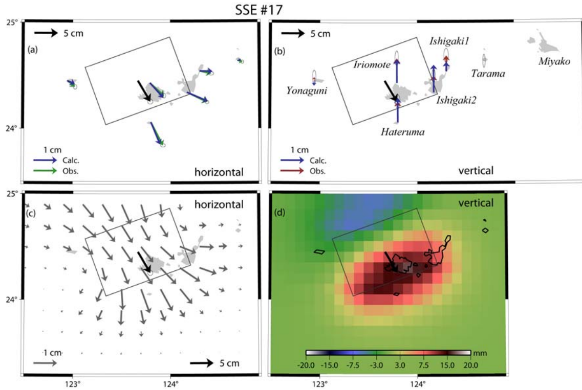
Fig.4 The estimation of the fault patch that moved in the 17 th SSE using the observed horizontal (green arrow in a) and vertical (red arrows in b) displacements. The fault patch is centered at (24°27'N 123°47'E) and at depth of 32 km, and its dimension is 94 km in length and 66 km in width. It dips 15° toward NNE with strike 250°. Blue arrows in (a) and (b) are the displacement vectors calculated using the fault slips shown by the black arrow. We used the model by Okada [1992]. Calculated horizontal and vertical displacements at grid points are given in (c) and (d), respectively.
