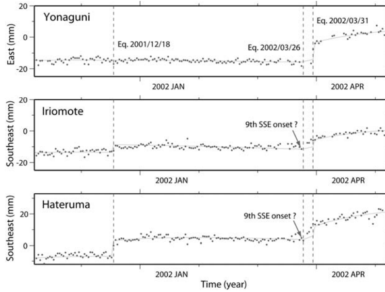
Fig. 9 Movements of three GPS stations from 2001 November to 2002 May relative to Miyako. Vertical dashed lines show the earthquakes in Fig.8. Yonaguni shows coseismic movements associated with the 2002 March 31 earthquake, but the other two stations do not. On the other hand, Iriomote and Hateruma show coseismic movements in the 2001 December 18 earthquake while Yonaguni does not. The 9 th SSE seems to have started simultaneously with the 2002 March 26 earthquake.
