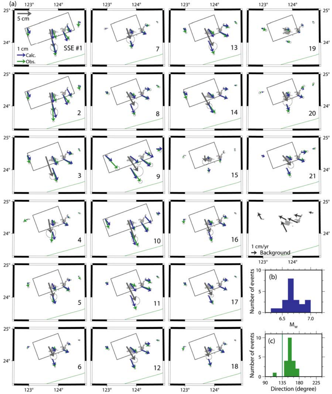
Fig.5 (a) Horizontal displacement vectors (blue/green arrows) and estimated fault slips (gray arrows) for the twenty-one SSE studied here. Error ellipses indicate 2\sigma . For SSE 1, 2, 9, and 10, we extended the fault length by 20 km in both directions. For SSE 3 and 14, the extension was done only toward WSW. For the other events, the same fault as in Fig. 4 is assumed. Below the panel for the 21 st SSE we show the background velocity vectors (black arrows) estimated as a in equation 1 (for the Yonaguni station, its time-averaged velocity shown in Fig. 1c is subtracted to isolate interseismic velocity). (b) Histogram showing the distribution of moment magnitudes. (c)
