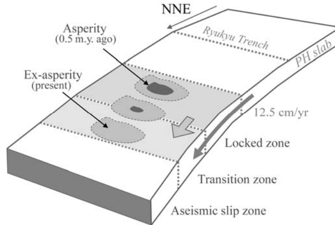
Fig. 10. An image of alteration of an asperity on the PH slab subducting beneath SR at the Ryukyu Trench. The strongly coupled unstable part (asperity, shown in dark gray) was surrounded by conditionally stable part (light gray) which was normally coupled but moved slowly following the fast rupture in the asperity. The unstable part became smaller as the slab subducted to a deeper part and ambient temperature increases. The unstable part eventually disappeared and the whole part slips episodically but aseismically now.
