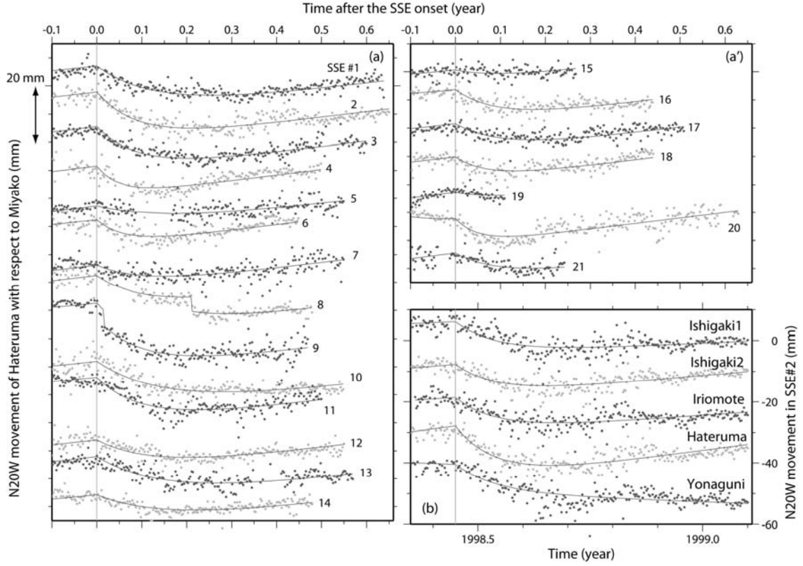
Fig.3 (a) The same time series as in Fig.2a (daily N20W displacements of Hateruma) are shown by plotting individual SSE separately with the origin at their onset times. Difference in the darkness of the gray symbols is for visual clarity. Gray curves are model curves based on equation 1. SSE numbers (Fig.2) are labeled on each event. (b) Daily N20W coordinates of five different GPS sites for the same SSE (2 nd ) are compared to show the coherence of movements at these sites. If the rupture propagated at a rate 6 km/day as in Cascadia [Dragert et al. , 2001], it would take \sim 2 weeks for the rupture to propagate between Ishigaki and Yonaguni (separated by \sim 100 km).
