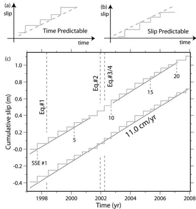
Fig. 7 If recurrences are time- (a) or slip-predictable (b), the lower-right or upper-left corners, respectively, of cumulative slip diagrams are expected to align. (c) Cumulative slip by the SSE
