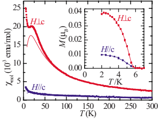
FIG. 2. (Color online) Temperature dependence of the magnetic susceptibility of TPP[Fe(Pc)(CN) 2 ] 2 . The inset shows the spontaneous magnetization measured at the zero field for the sample cooled in the field of 55 kOe. The solid lines show the calculations of magnetic susceptibility based on the anisotropic Heisenberg model [Eq. (1)]. See the details in Sec. IV.
