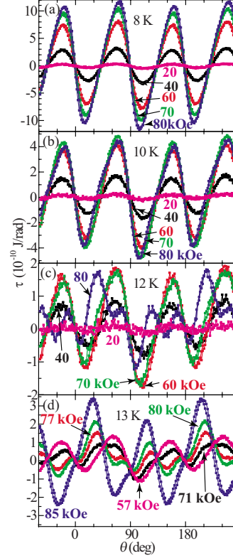
FIG. 6. (Color online) Magnetic torque curves of \text{TPP}[\text{Fe}(\text{Pc})(\text{CN})_2]_2 below T=13 K. Note the complicated structures of the torque curves at 12 and 13 K before the T_1 inversion.
