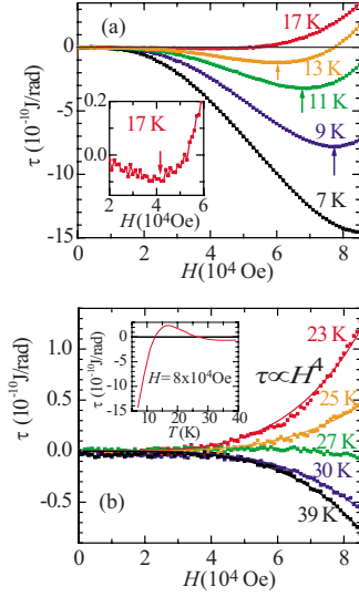
FIG. 5. (Color online) Field dependences of the magnetic torque of \text{TPP}[\text{Fe}(\text{Pc})(\text{CN})_2]_2 at \theta=22.5^\circ (a) below T=17 K and (b) above T=23 K. The data below 17 K exhibit a minimum, followed by an inversion. On the other hand, no inversion is observed above 23 K. The arrows in (a) indicate the minimum of the curve. The solid lines in (b) indicate the fit of \propto H^4 to the experimental data. The insets (a) and (b) show the torque minimum at 17 K and the temperature dependence, respectively.
