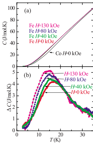
FIG. 8. (Color online) (a) Heat capacity of \text{TPP}[M(\text{Pc})(\text{CN})_2]_2 ( M=\text{Fe}, \text{Co} ). (b) The difference in the heat capacity between the two compounds ( \Delta C ). The magnetic field enhances the \Delta C .
