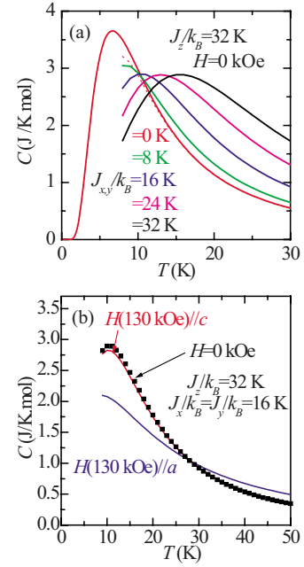
FIG. 12. (Color online) (a) Calculations of the heat capacity based on the anisotropic Heisenberg model in one dimension. The calculations at J_{x,y}=0 are the results of an exact solution based on the Ising model. The red dotted line indicates the results of the numerical calculation for the same Ising model. (b) The calculation of the heat capacity under the applied magnetic field for the anisotropic Heisenberg model ( J_z/k_B=32 K; J_{x,y}/k_B=16 K). The squares indicate the calculations at the zero field. The heat capacity is seriously depressed for H\parallel a , but it is almost unchanged for H\parallel c .
