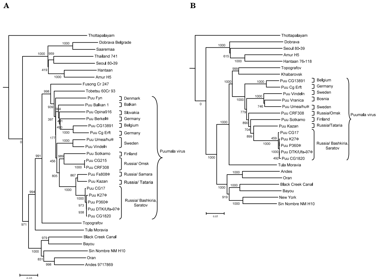
Fig. 3. Phylogenetic analysis of hantaviruses.
