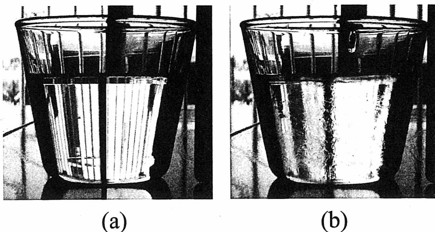
Figure 1: (a) Pure fluid; (b) Binary fluid. Scenery is distorted due to the spatial fluctuation of concentration field of alcohol.
