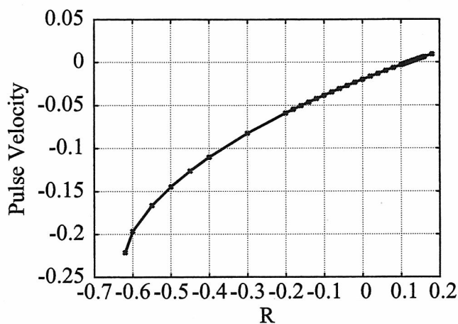
Figure 4: Pulse velocity of a pulse. Pulse solution exists in the region -0.62 \leq R \leq 0.18 . Depending on R , the velocity can be both positive and negative.
