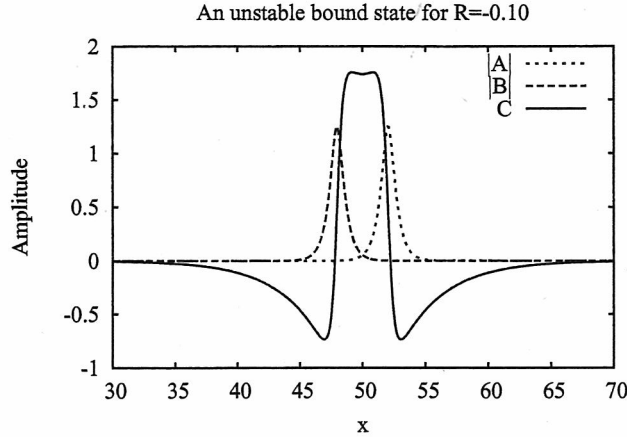
Figure 10: An unstable time-periodic bound solution obtained by the delayed feedback control method.
