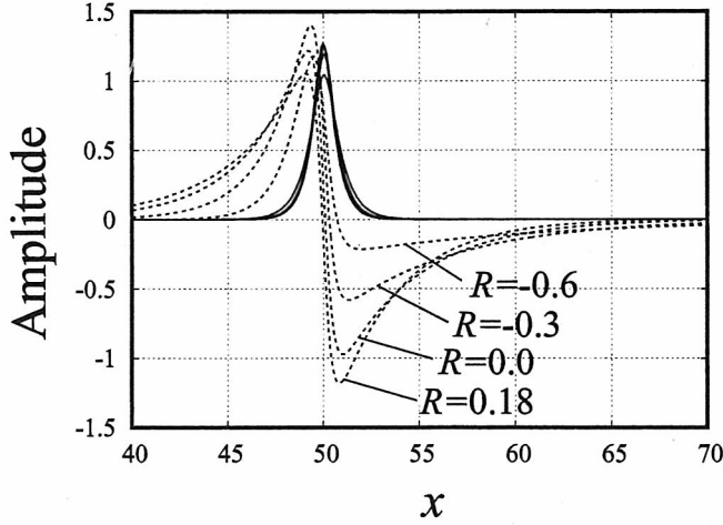
Figure 3: Pulse solutions. Solid line stands for the amplitude of A , and broken line for C .
