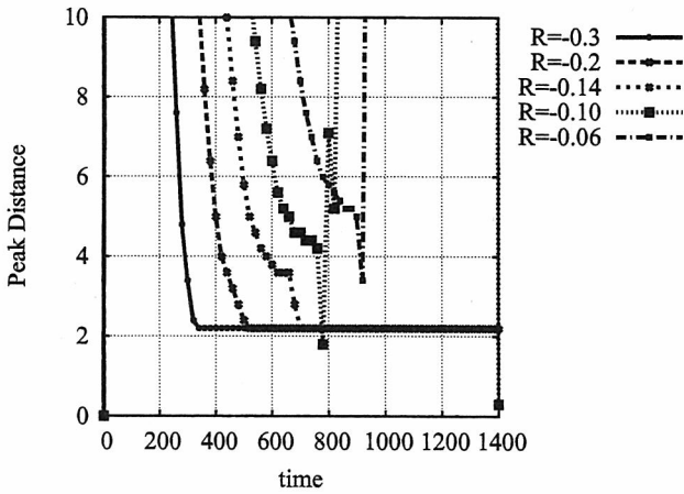
Figure 9: The distance of pulses during the collision process. We can see quasi-steady states for R = -0.14(600 \leq t \leq 650) and for R = -0.10(t \simeq 750) .
