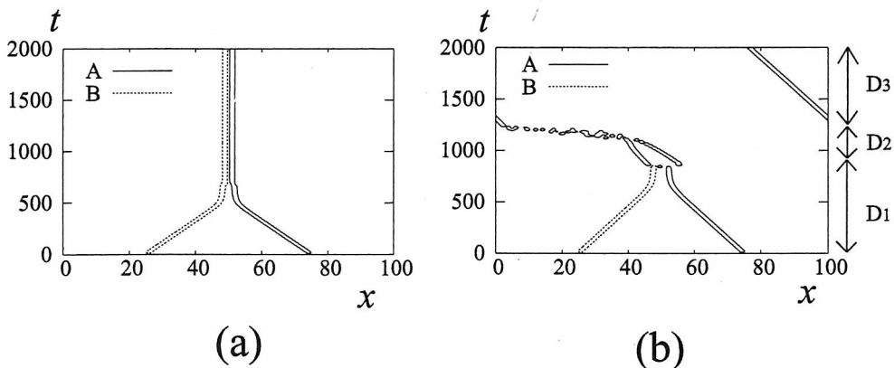
Figure 6: (a) Space-time plot of pulse collision for R = -0.14 . Contours of |A| (solid line) and |B| (dotted line) are shown. Asymptotic state is a bound state. (b) Space-time plot of pulse collision for R = -0.08 . Two pulses come close to each other ( D_1 ). Due to strong interaction, one pulse annihilates. A new order is constructed during the interaction ( D_2 ), but only one pulse survives asymptotically ( D_3 ).
