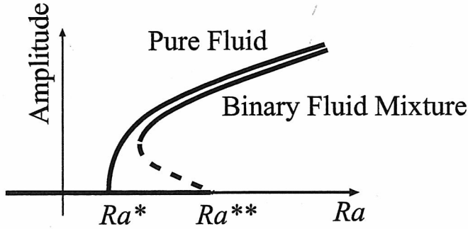
Figure 2: Schematic Picture of the bifurcation diagram in Rayleigh-Benard convection. Supercritical bifurcation causes convective flow for pure fluid, while subcritical bifurcation for binary fluid mixture.
