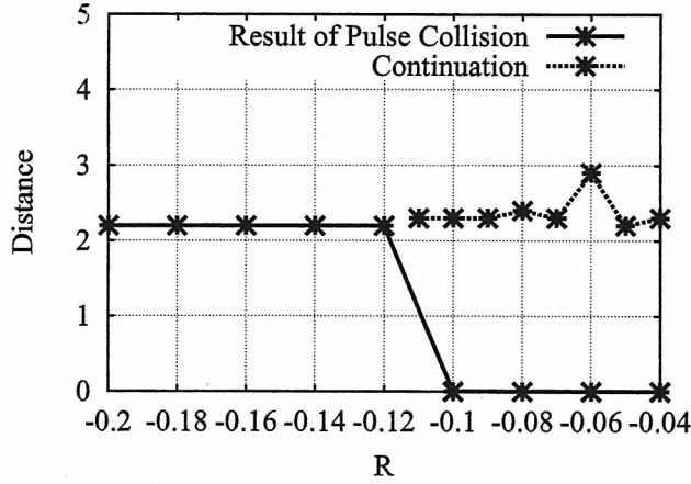
Figure 8: The distance of bound state. Solid line shows the asymptotic state of pulse collision, which is destruction state in the region -0.1 \leq R \leq -0.04 . Dotted line shows the asymptotic states by continuation starting from the bound state at R = -0.12 .
