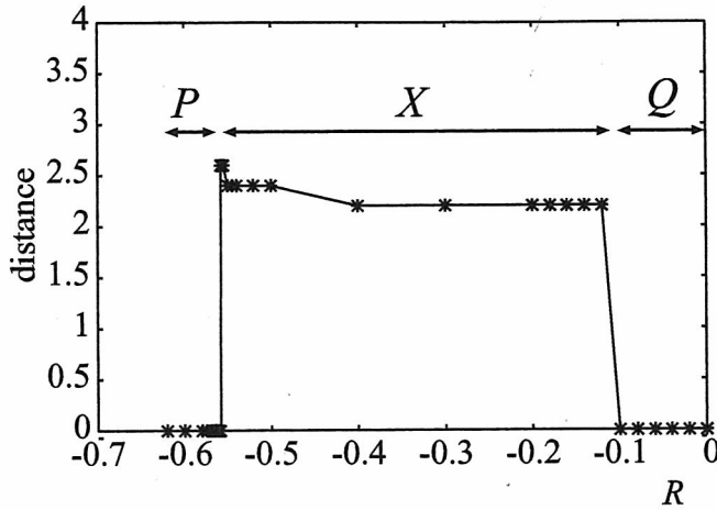
Figure 7: The result of the pulse collision. If bound state is formed as a result of pulse collision (region X ), the distance of the bound state is shown. Destruction state is obtained in the region P and Q .
