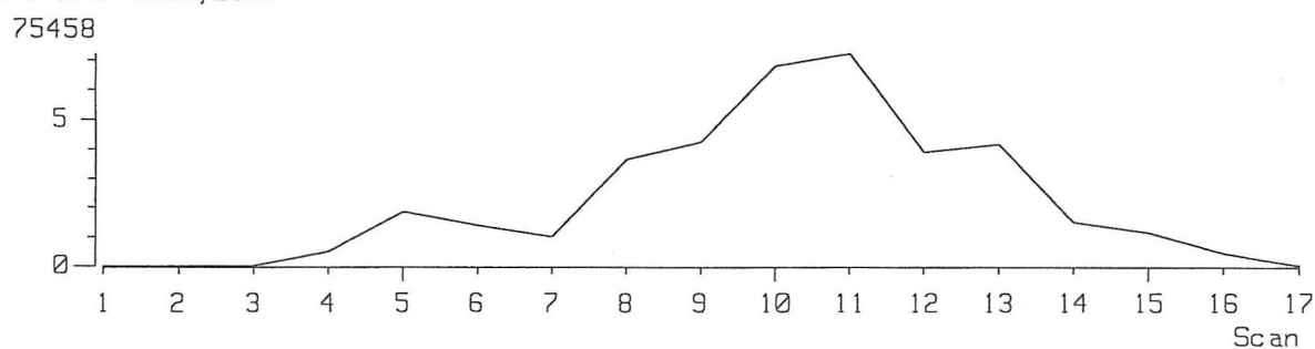
[ Mass Chromatogram ]
