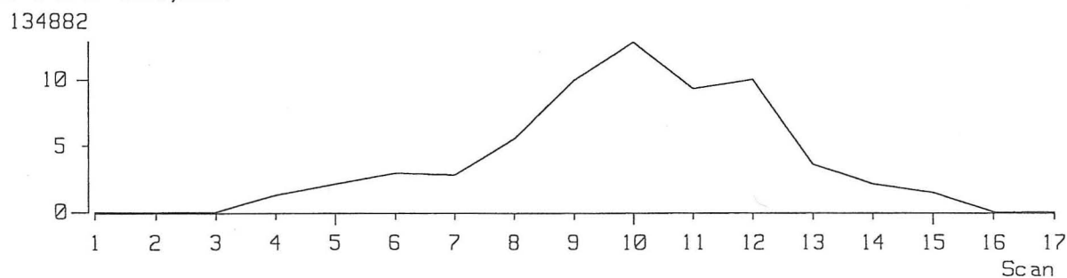
[ Mass Chromatogram ]
