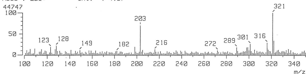
[ Mass Chromatogram ]
