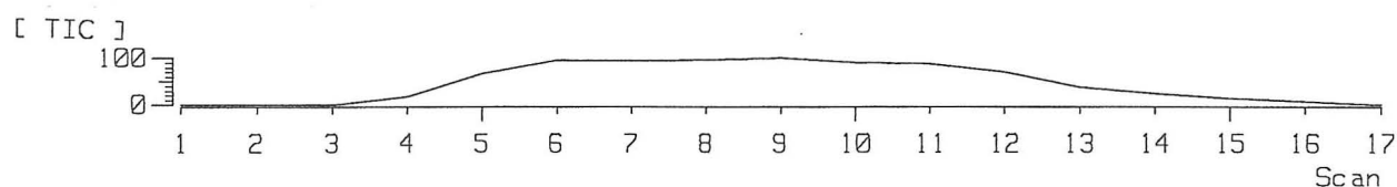
[ Mass Spectrum ]
