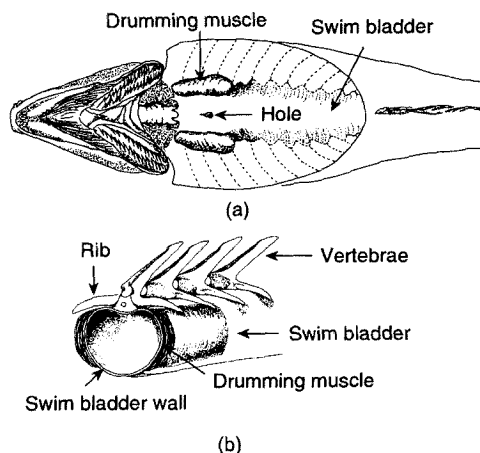
Fig. 1. Mechanisms of the sound-producing organ: (a) Ventral view of swim bladder; (b) Transversal view of swim bladder at the level of the drumming muscles.
