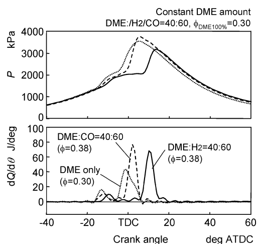
Fig. 7 Ignition control effects by additions of hydrogen and carbon monoxide to HCCI combustion of DME at constant DME amounts
