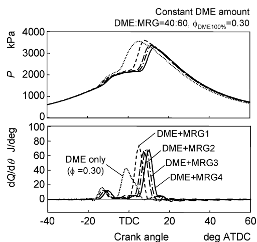
Fig. 6 Ignition control effects by addition of the MRG to HCCI combustion of DME at constant DME amounts
