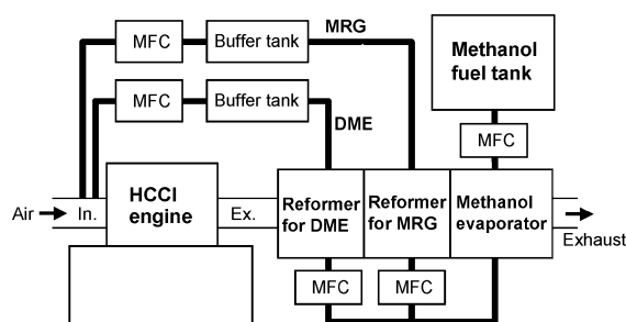
Fig. 1 Concept of the HCCI combustion engine system fuelled with DME and MRG onboard reformed from methanol
