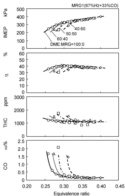
Fig. 4 i.m.e.p., indicated thermal efficiency, and exhaust emissions in HCCI combustion of DME and MRG1
