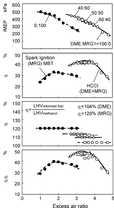
Fig. 14 Overall thermal efficiency
