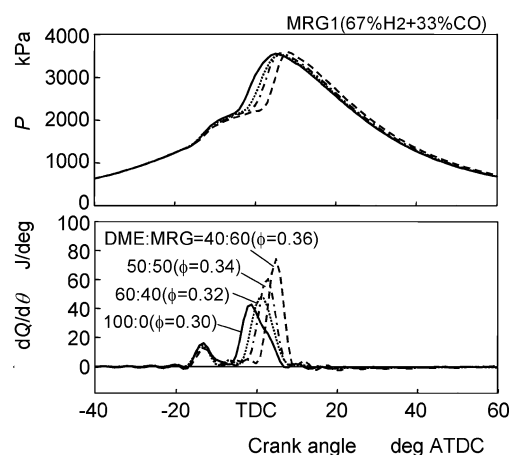
Fig. 5 Indicator diagrams for HCCI combustion of DME and MRG1 at optimum equivalence ratios for thermal efficiency
