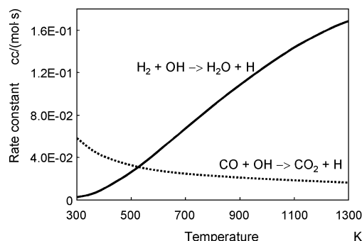
Fig. 8 Rate constants for \text{H}_2 + \text{OH} and \text{CO} + \text{OH}
