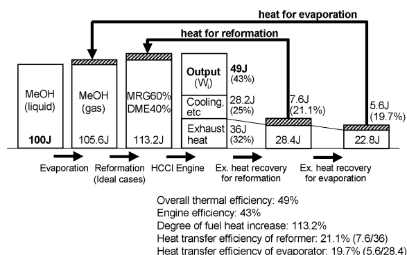
Fig. 15 Typical example of heat balances
