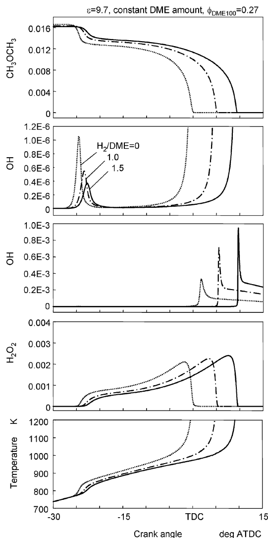
Fig. 9 Calculated mole fraction of species and temperature in DME HCCI combustion with different hydrogen fractions
