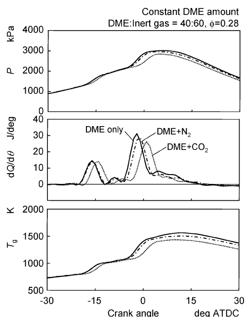
Fig. 11 Influence of heat capacity of mixture on HCCI combustion of DME
