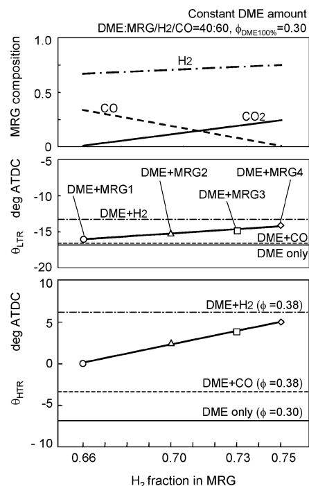
Fig. 10 Influence of MRG composition on the onsets of the low and high-temperature oxidation reactions in HCCI combustion of DME
