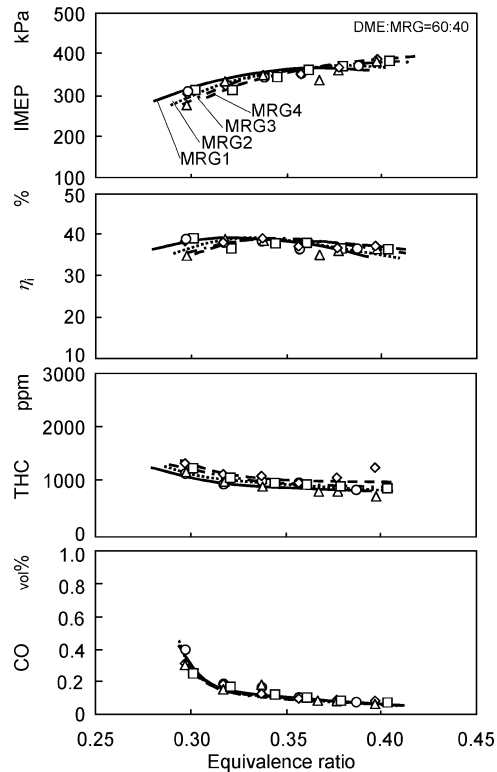
Fig. 12 HCCI combustion of DME and the four types of MRG
