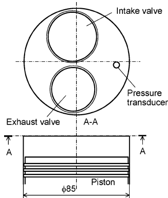
Fig. 3 Combustion chamber of the tested engine
