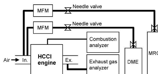
Fig. 2 Experimental system using model gases
