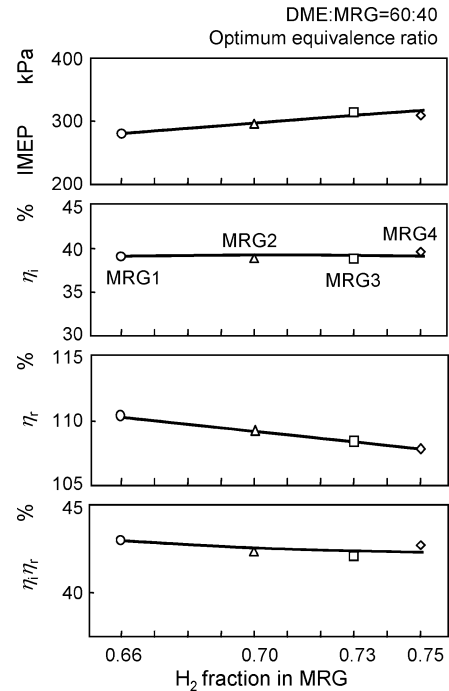
Fig. 13 Influence of MRG composition on the overall thermal efficiency including heat recovery through methanol reforming
