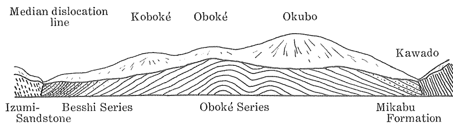
Fig. 3. Ideal section along the Oboké Valley.
