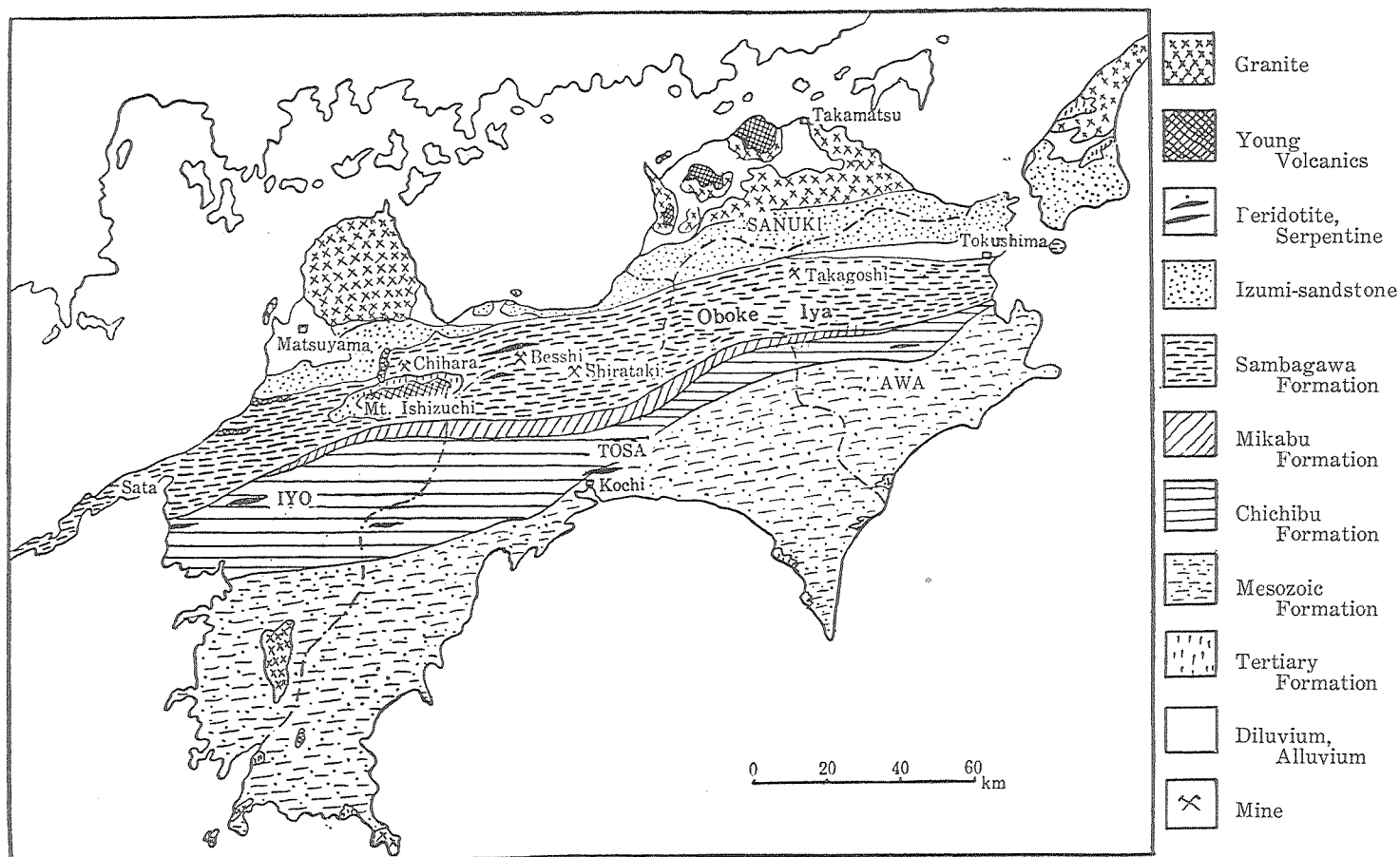
Fig. 1. Geological Map of Shikoku.
