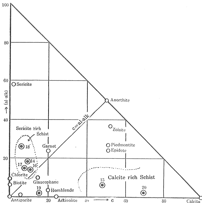
Fig. 12. al, alk-Diagram (siliceous and calcareous schists).
