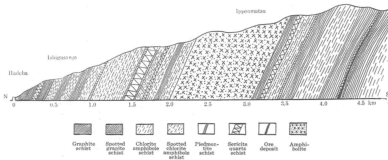
Fig. 4. Profile along the Fourth Tunnel of the Besshi Mine.
