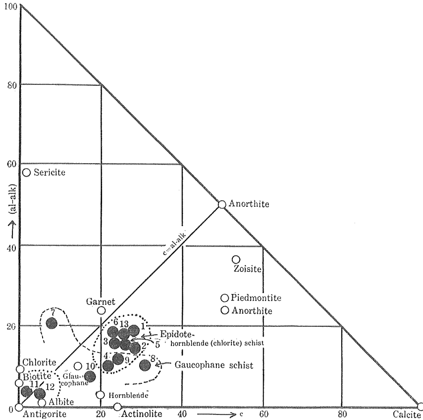
Fig. 9. (al-alk), c-Diagram (green schists).
