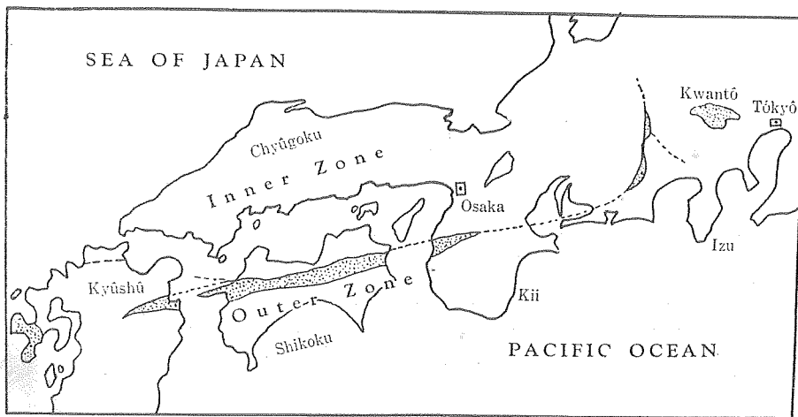
Fig. 2. Map, showing the distribution of the Crystalline Schist System of Japan.
