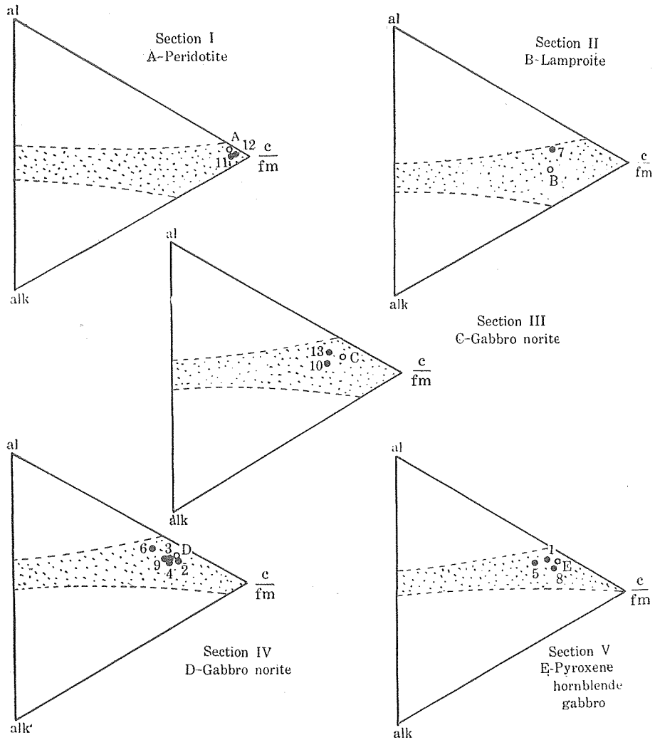
Fig. 8. al, alk, c/fm-Diagram.
