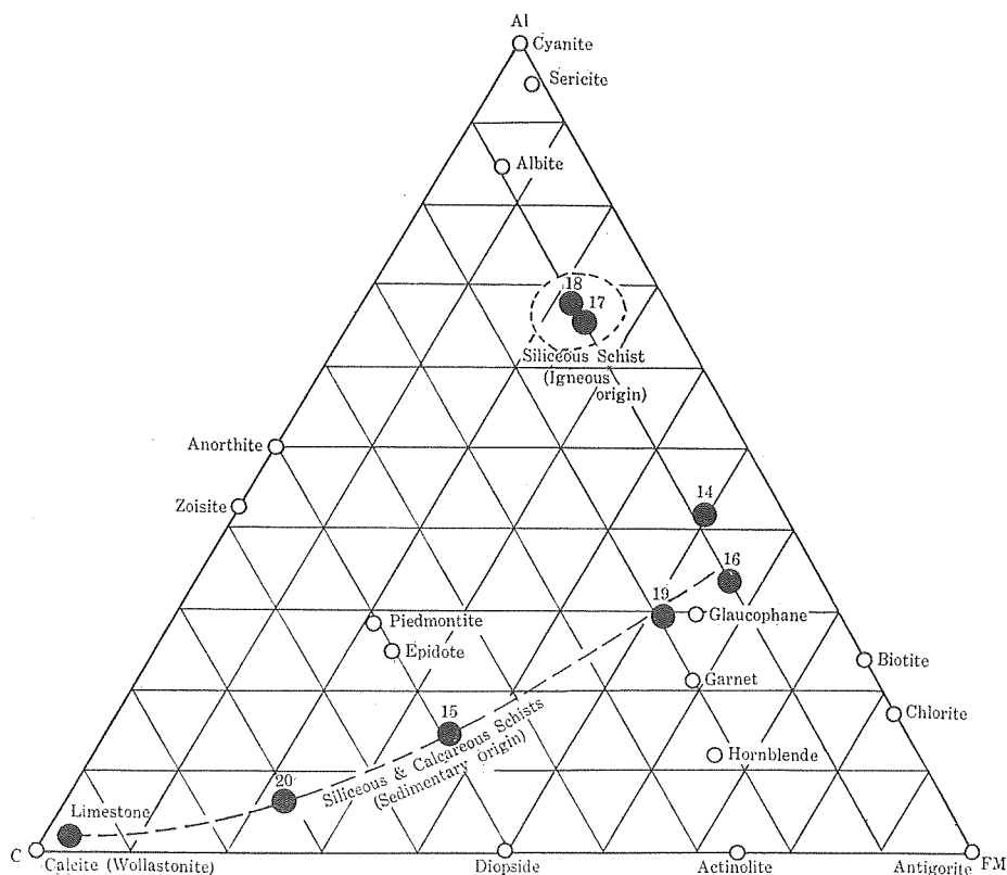
Fig. 13. AL-FM-C-Diagram (siliceous and calcareous schists).
