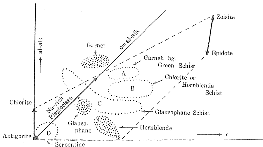
Fig. 10. (al-alk), c-Diagram (green schists).
