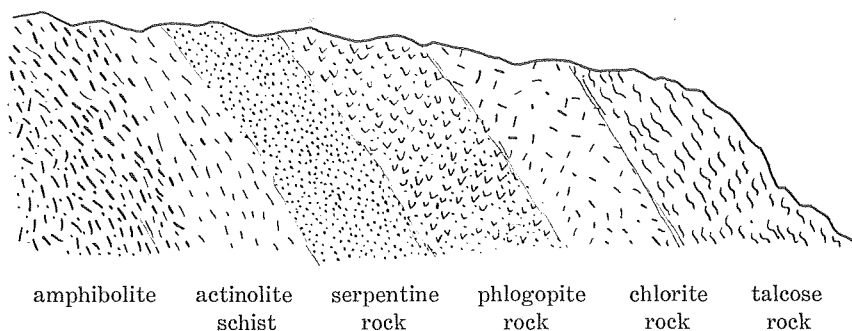
Fig. 5. Ideal section of the marginal part of the amphibolite mass.
