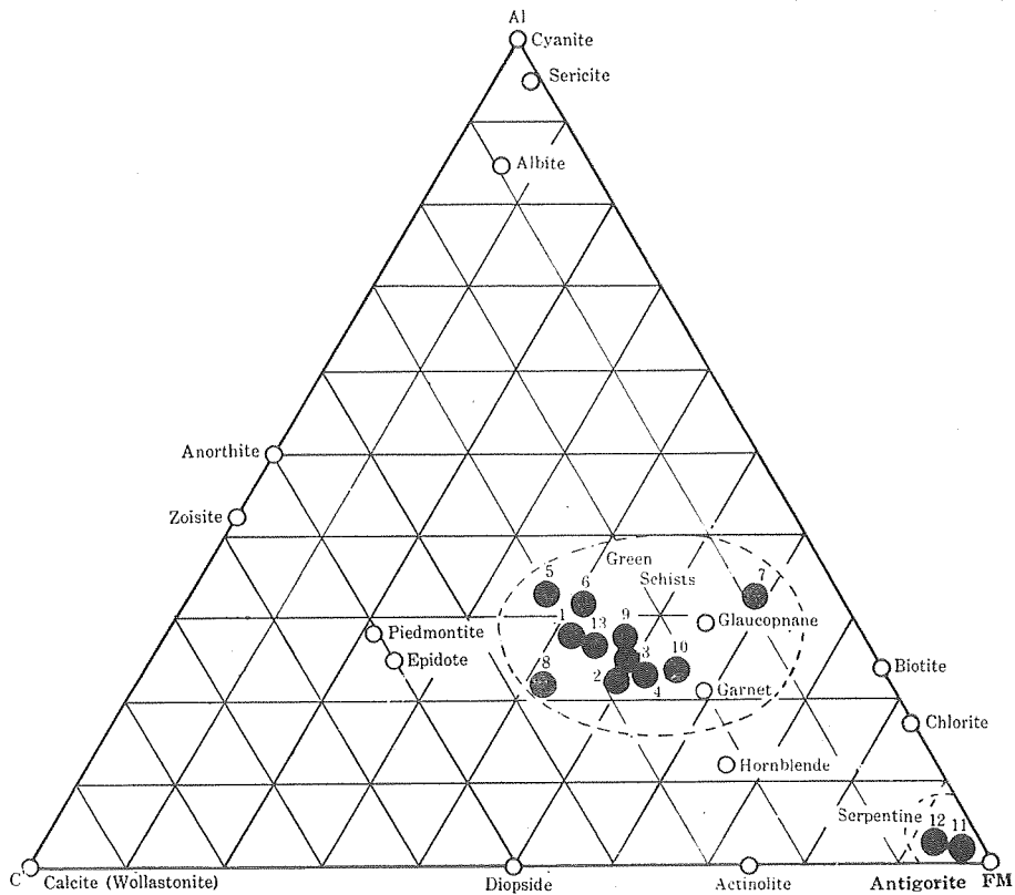
Fig. 11. AL-FM-C-Diagram (green schists).
