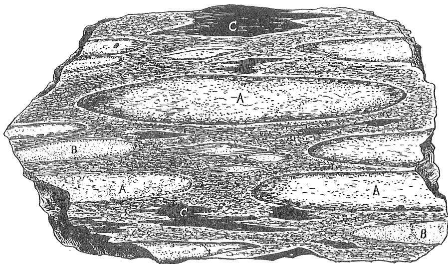
Fig. 6. Conglomerate schist from the Iya Valley in Shikoku 1/3 nat. size.
