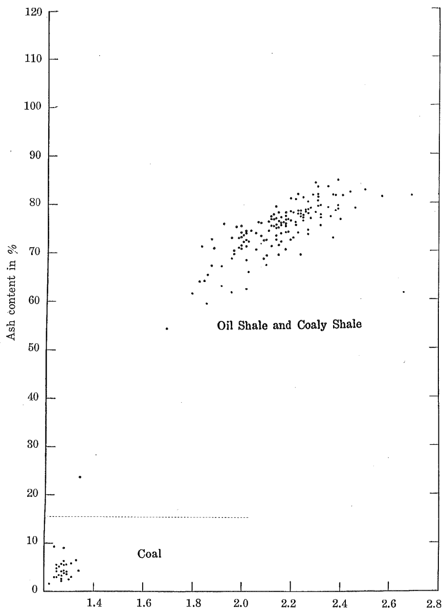
Fig. 19. Specific gravity.
