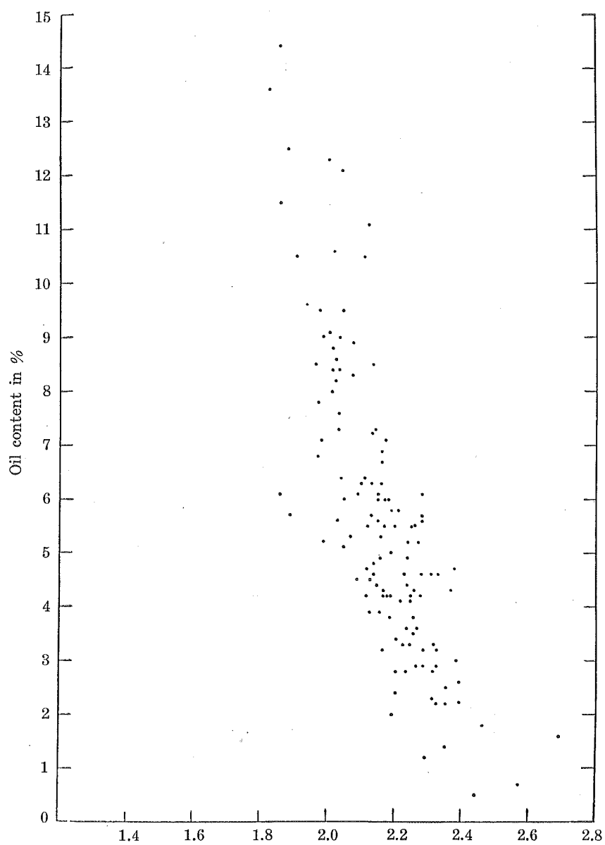
Fig. 18. Specific gravity.
