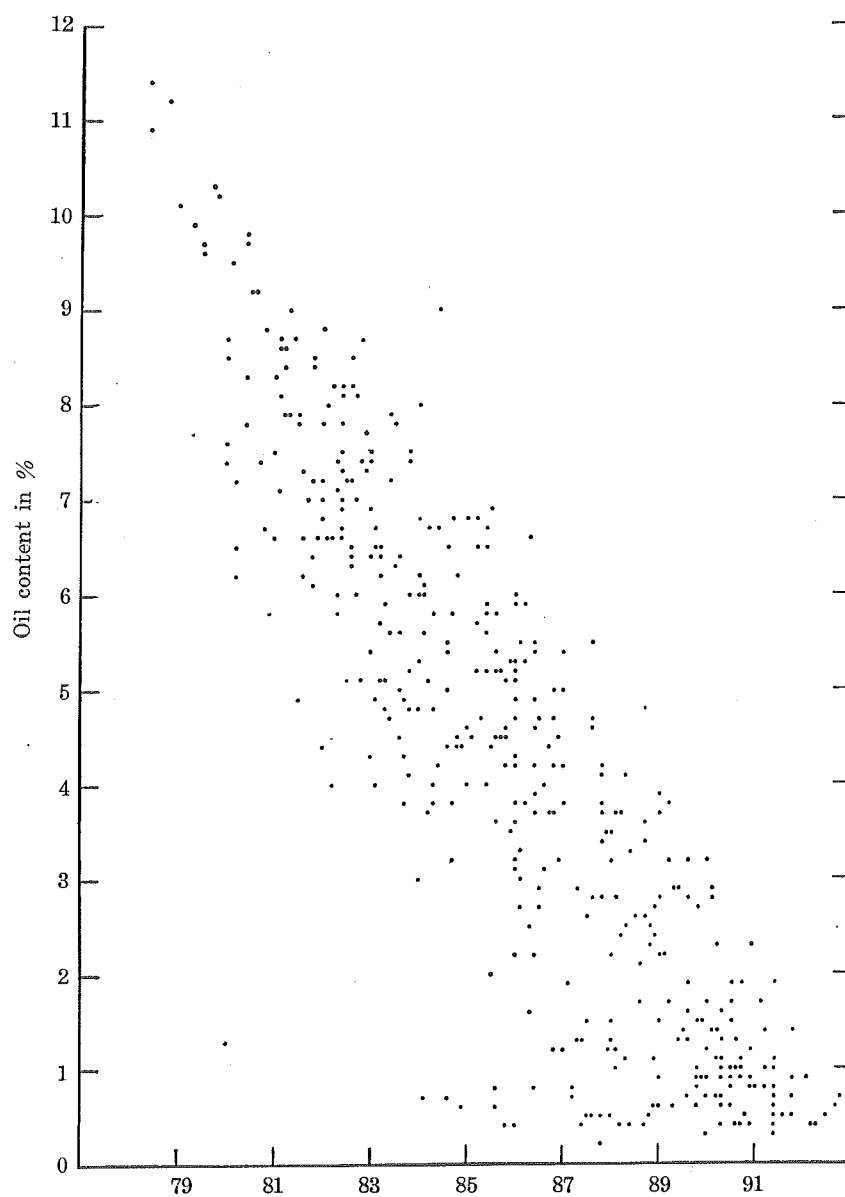
Fig. 14. Residue in %
