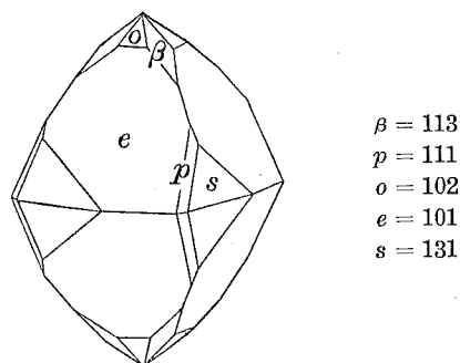
Fig. 8. Crystal of scheelite from the Sanjō mine. (1)
