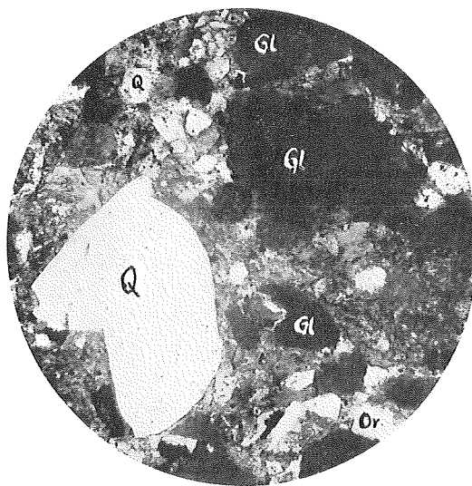
Figure 4. Glauconite Sandstone ( \times 65 ). Q, Quartz. Or, Orthoclase. Gl, Glauconite.
