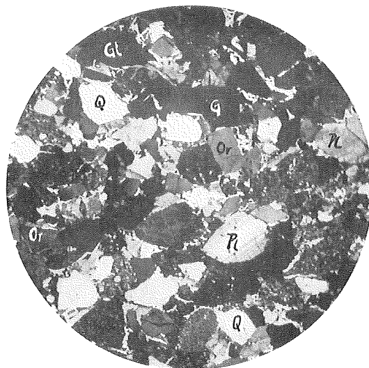
Figure 3. Typical sandstone of the Lower Hetonai Group (+Nicol. \times 60 ).
