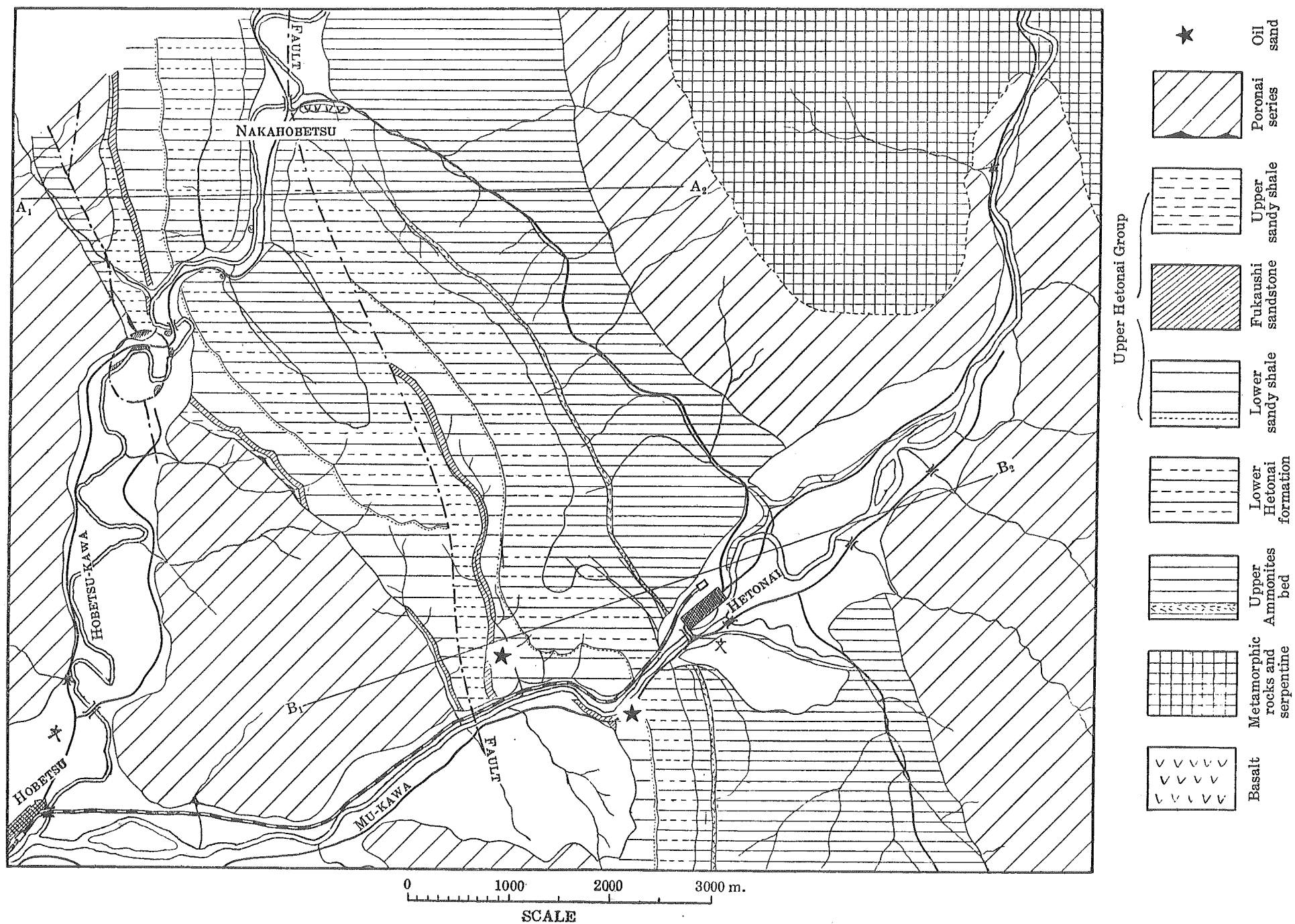
Figure 1. Geological Map of the Hetonai District.
