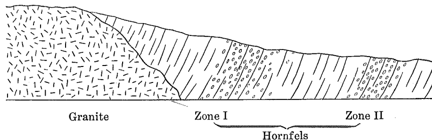
Fig. 3. Diagrammatic sketch showing the relationship between the granite and the concretion bearing hornfels. In zone I the concretion is highly recrystallized and has a very thick marginal shell, while in zone II it is less metamorphosed and has a thinner marginal shell.
