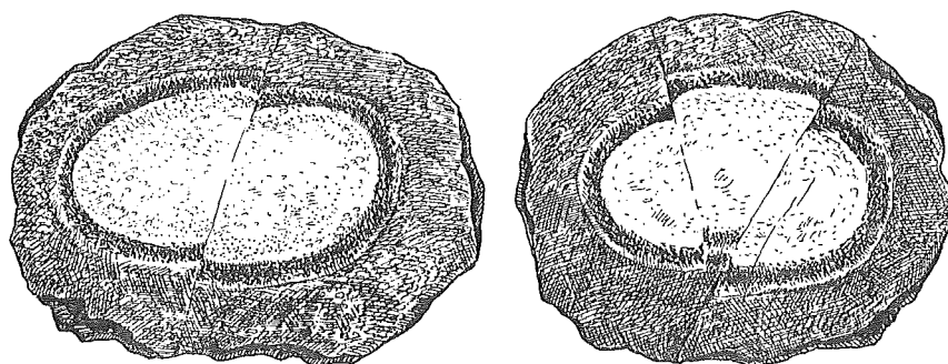
Fig. 2. Nodules traversed by minor faults. \frac{1}{2} nat. size.
