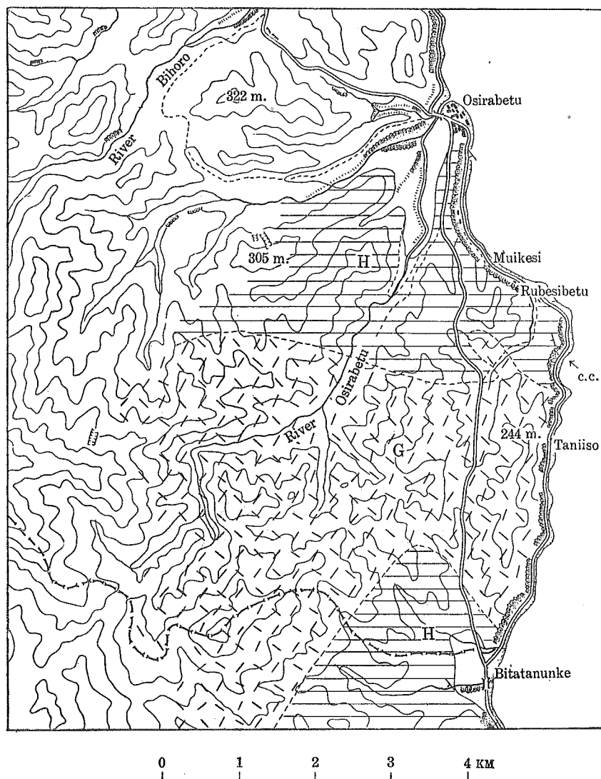
Fig. 1. Sketch map to show the geology of the Osirabetu district, Prov. Tokati. G : Granite, H : Hornfels, C. C : Calcareous concretions.
