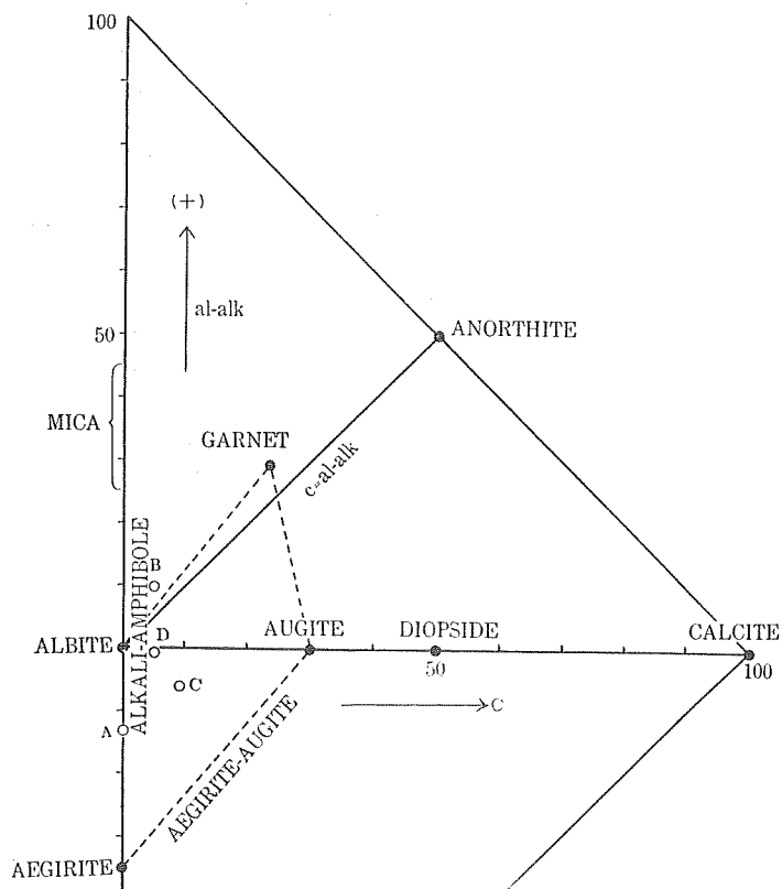
Fig. 5. c-(al-alk) diagram.
