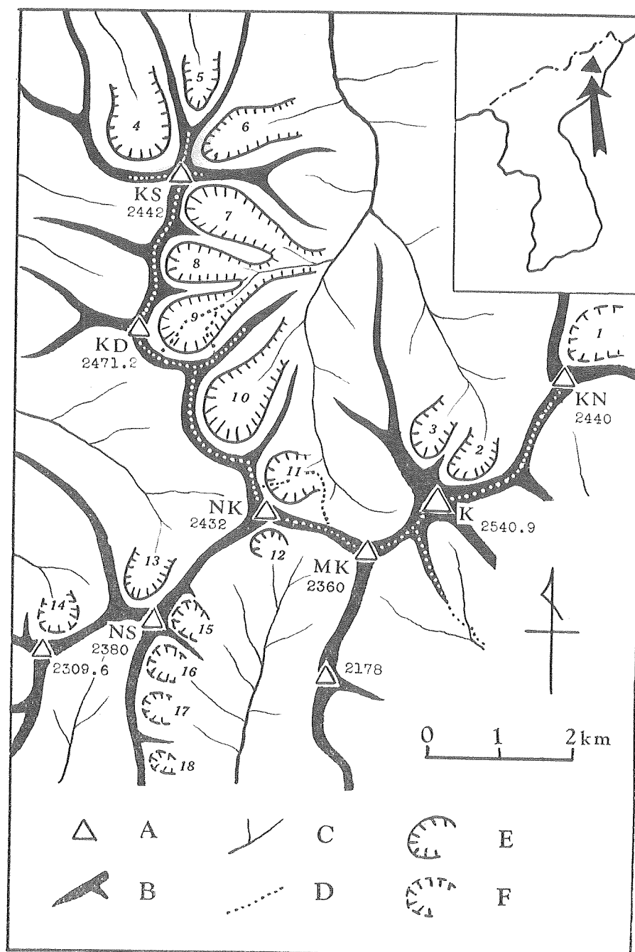
Fig. 2. Map showing the distribution of the glacial topography in the Kanbô Massif.
