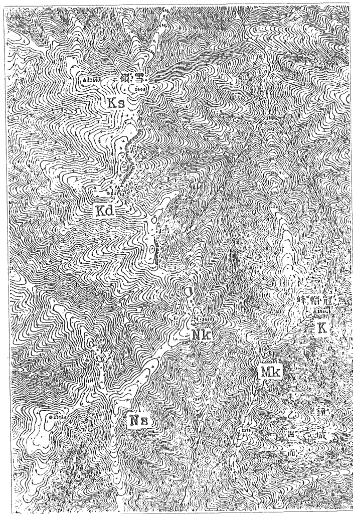
Fig. 1. Topographical map of the main part of the Kanbô Massif. The wide flat-topped ridges are well represented. The cirques are indistinctly drawn. (Scale; 1 : 75000. Contour interval : 20m. Reproduced from sheet Kanbôhō. 1 : 50000, Military Survey Map.)
