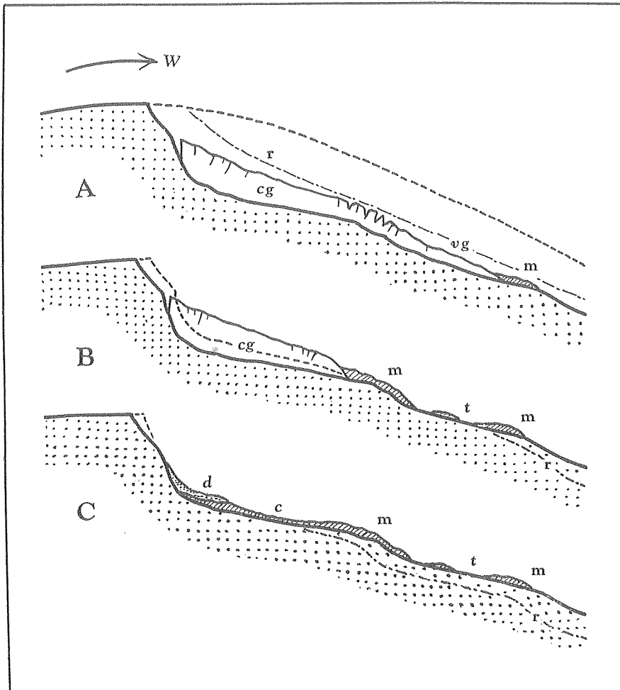
Fig. 11. Diagrammatic explanation to illustrate the stages of development of glacial sculpture on the Kanbô Massif.
