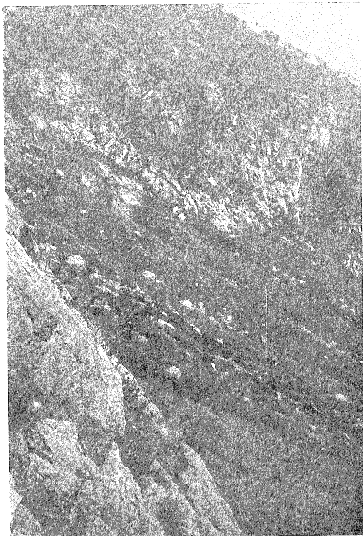
Fig. 10. Slabs at the foot of cirque wall in cirque No. 11. The foot of the wall is thickly buried under talus-cones. (Photo. by Y. Sasa)
