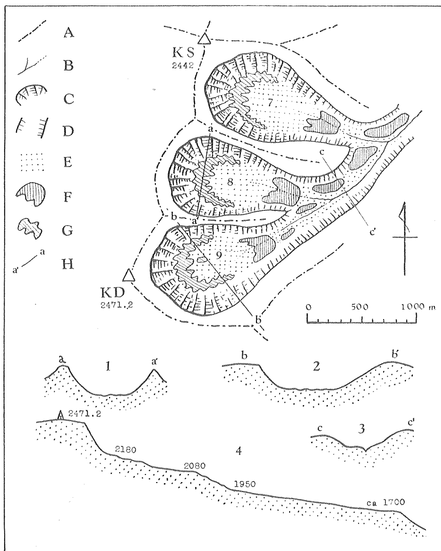
Fig. 3. Sketch map of cirques Nos. 7, 8 and 9.
