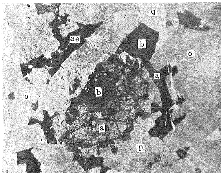
Fig. 2. Rock of nordmarkitic composition. \times 17 , o: orthoclase, p: albite, q: quartz, b: barkevikite, a: aegirine, ae: aenigmatite.
