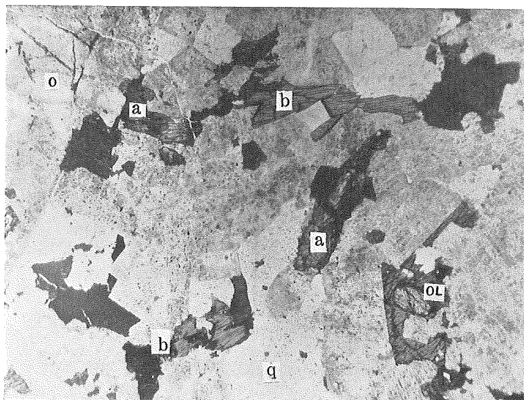
Fig. 1. Rock of nordmarkitic composition. \times 22 , o: orthoclase, q: quartz, b: barkevikite, a: aegirine, ol: fayalite.
