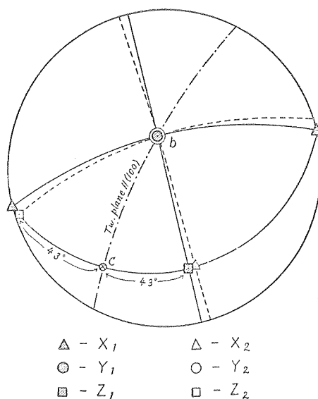
Fig. 3. Stereographic projection of optical elements of two twinned individuals.
