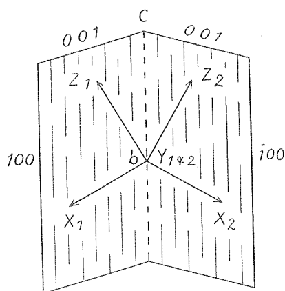
Fig. 1. Crystallographic and optic orientations of monoclinic twinned crystal on (010).
