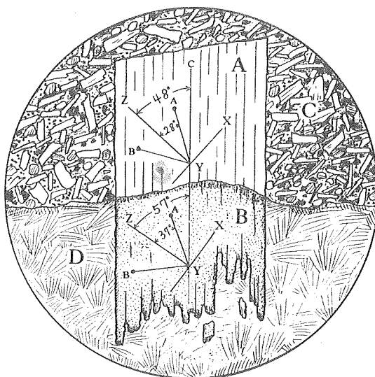
Fig. 2. Diagrammatic sketch of the crystal, parallel to (010), showing an intergrowth of common augite (A) and aegirine-augite (B).
