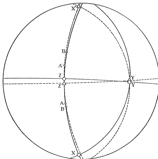
Fig. 3. Stereogram showing the relation between common augite and aegirine-augite. Full line and circle for common augite, and dotted line and triangle for aegirine-augite.
