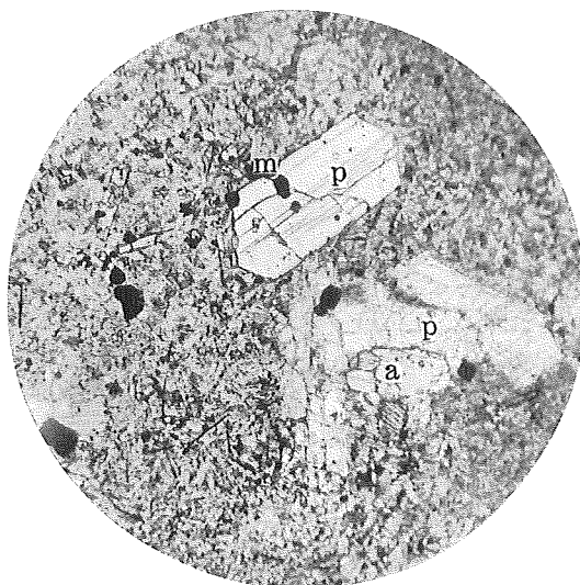
Fig. 1. Analcime dolerite from Bentenzima near Nemuro. ×22, p: plagioclase (labradorite-bytownite) a: analcime, m: magnetite.
